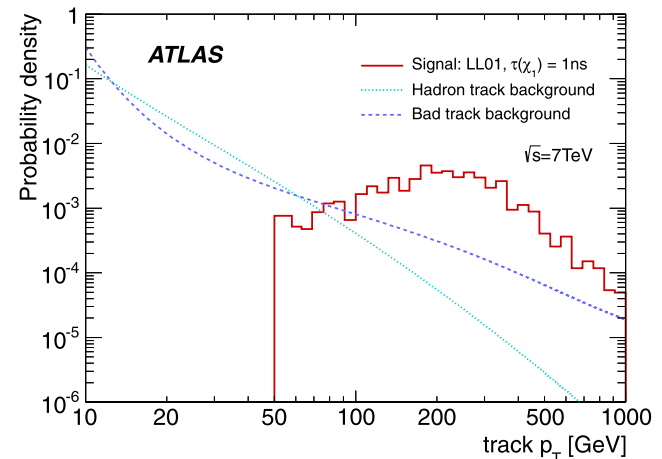
Fig. 4 Probability densities of the signal (LL01, \tau_{\chi_{\pm 1}} = 1 ns) and background components, shown as a function of track p_T . In the signal case, only the region p_T > 50 GeV is shown
