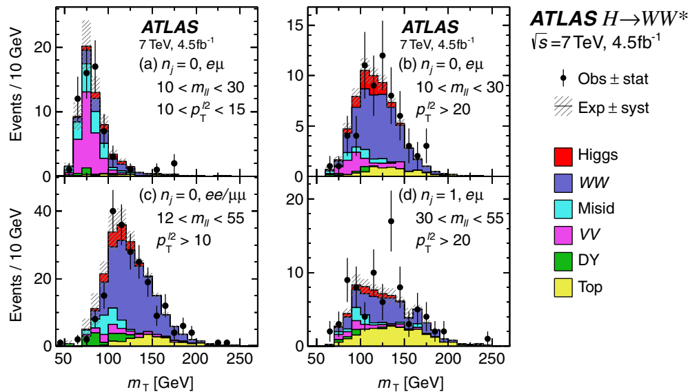
FIG. 34 (color online). Postfit transverse mass distributions in the n_j \leq 1 categories in the 7 TeV data analysis, for specific m_{\ell\ell} and p_T^{\ell 2} ranges. The plots are made after applying all the selection requirements (see Sec. IV E). See Figs. 5 and 29 for plotting details.
