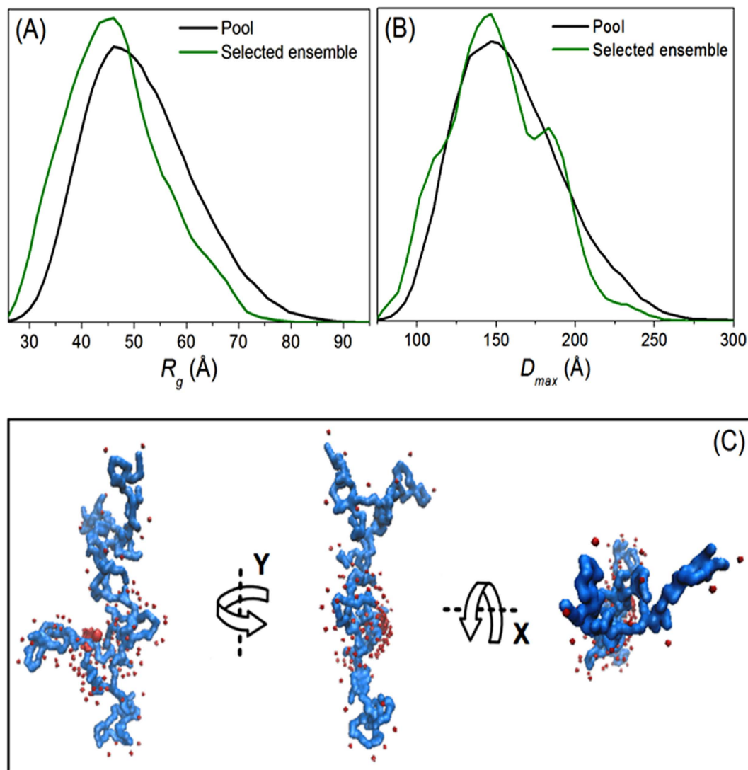
Figure 4. (A) Radius of gyration ( R_g ) and (B) Maximum particle size ( D_{max} ) distributions of Rec1-resilin plotted as functions of frequency (arb. unit) using the ensemble optimization method (EOM). (C) Representative ab initio 3D-model structure (one among an infinite ensemble of possible 3D-densities) of Rec1-resilin reconstructed using the GASBOR program from the distance distribution function output.
