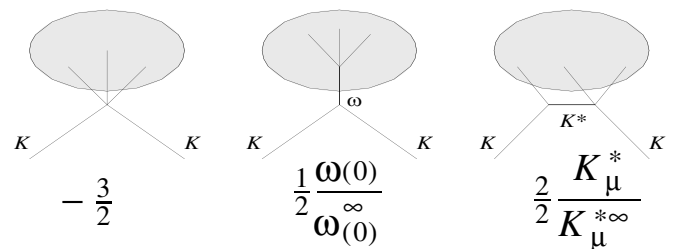
FIG. 1. Schematic illustration of the WZ-like terms due to vector mesons in the Lagrangian (7). The baryon number density is given by the three pion lines stemming from the shaded area, i.e., the soliton. In the limit of infinitely heavy meson masses, an exact cancellation takes place among the three terms.
