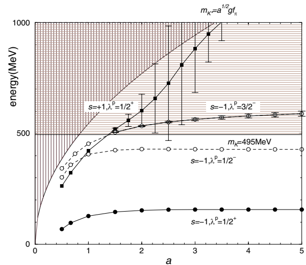
FIG. 2 (color online). The eigenenergies of S = \pm 1 , \lambda^P = \frac{1}{2}^\pm, \frac{3}{2}^\pm states obtained for various a values. The width of the resonance in the K^+ -skyrmion channel is given by the error bar.
