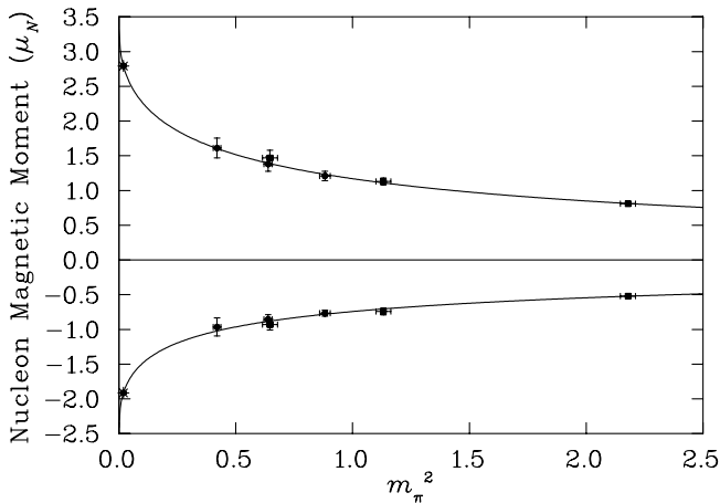
FIG. 1. Extrapolation of lattice QCD magnetic moments (•, LDW [8]; ■, WDL [9]) for the proton (upper curve) and neutron (lower curve) to the chiral limit. The curves are constrained to pass through the experimentally measured moments which are indicated by asterisks.
