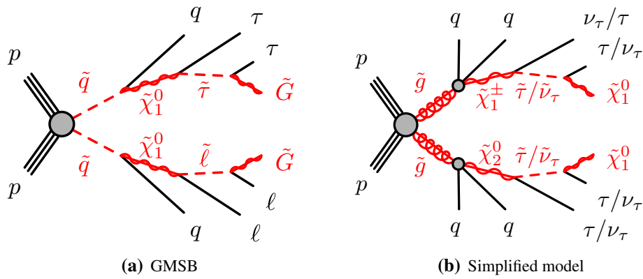
Fig. 1 Diagrams illustrating the two SUSY scenarios studied in this analysis. In the GMSB model, the scalar lepton \tilde{\ell} is preferentially a scalar tau \tilde{\tau}_1 for high values of \tan \beta
