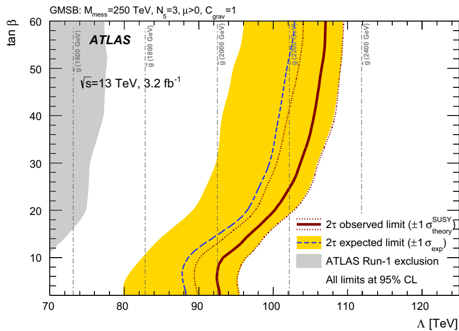
Fig. 9 Exclusion contours at the 95% confidence level for the gauge-mediated supersymmetry-breaking model, based on results from the 2\tau channel. The red solid line and the blue dashed line correspond to the observed and median expected limits, respectively. The yellow band shows the one-standard-deviation spread of expected limits around
