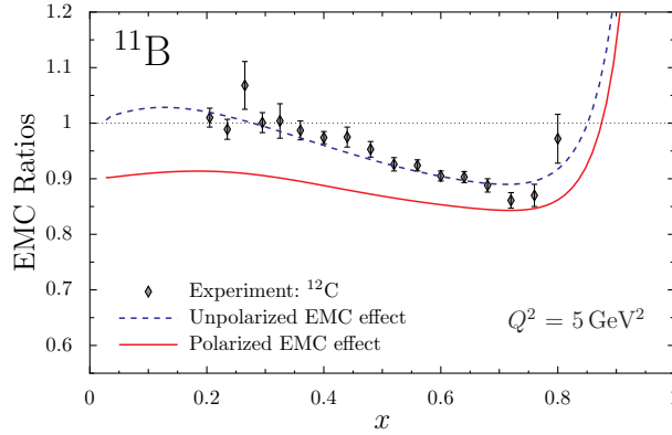
Figure 2: EMC ratios for the nucleus 11 B from Ref.[4]. The experimental data for 12 C are from Ref.[8].
