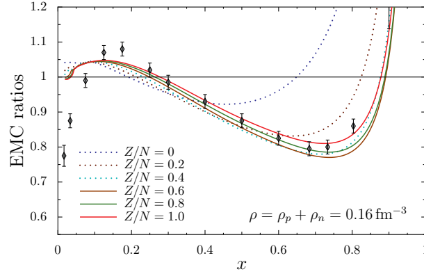
Figure 3: Spin independent EMC ratios for infinite matter at fixed baryon density for several ratios Z/N . The data points are the extrapolations of nuclear DIS to the limit of isospin symmetric nuclear matter[10].
