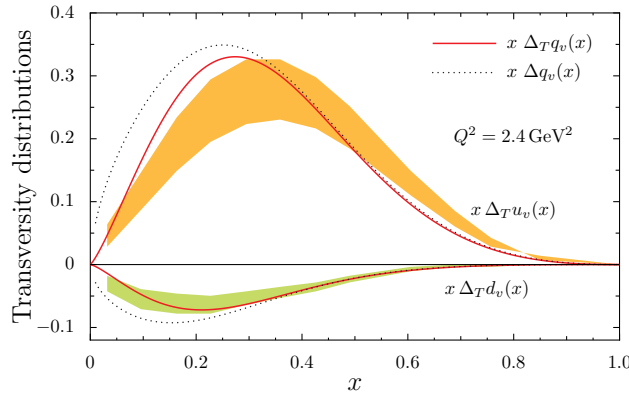
Figure 1: Calculated transversity quark distributions (solid lines, from Ref.[5]) in comparison to recent fits to data (shaded areas, from Ref.[6]). The dotted lines show the calculated helicity distributions for comparison.
