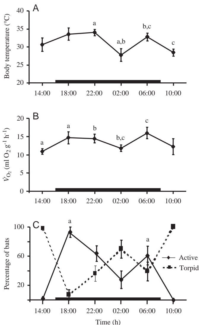
Fig. 1. Diurnal changes in (A) body temperature, (B) metabolic rate ( \dot{V}_{\text{O}_2} ) and (C) percentage of the bat colony observed as either torpid or warm-active for Nyctophilus geoffroyi at an ambient temperature, T_a , of 24^\circ\text{C} . Bats observed as 'torpid' were motionless, curled up and slow to respond to human touch. Those observed as 'warm-active' were alert and/or flying. The horizontal dark bars represent the period of darkness. Identical letters indicate points that are significantly different at P \leq 0.05 . Values are means \pm S.E.M.; N=5-6 for each point in A and B, and N=36 for each point in C.
