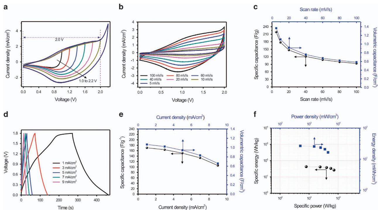
Figure 7 (a) CV curves for MnO 2 //FeCo 2 O 4 asymmetric SCs device at different potential range ranging from 1.0 to 2.2 V, (b) CV curves for MnO 2 //FeCo 2 O 4 asymmetric SCs device at different scan rate within operating potential range of 0-2.0 V, (c) the plot of specific and volumetric capacitance versus scan rate for MnO 2 //FeCo 2 O 4 asymmetric SCs device, (d) the charge-discharge curves for MnO 2 //FeCo 2 O 4 asymmetric SCs device at various current density, (e) the plot of specific and volumetric capacitance versus current density for MnO 2 //FeCo 2 O 4 asymmetric SCs device and (f) the Ragone plot for the plot of specific and volumetric capacitance versus scan rate for MnO 2 //FeCo 2 O 4 asymmetric SCs device.
