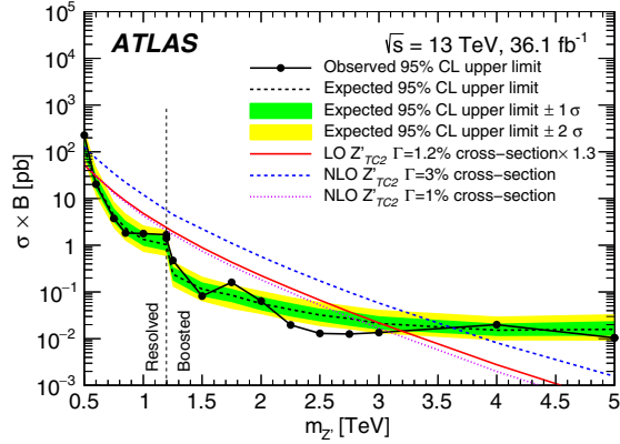
FIG. 9. Observed and expected upper limits on the cross-section times branching fraction of Z'_{TC2} decaying into t\bar{t} as a function of the Z'_{TC2} mass. The theory predictions of the cross sections for the Z'_{TC2} with \Gamma = 1\% and 3\% are shown by the dotted and dashed lines at NLO and by the solid line with \Gamma = 1.2\% at LO, respectively. The results from the resolved and boosted analyses are shown to the left and right of the vertical dashed line, respectively.
