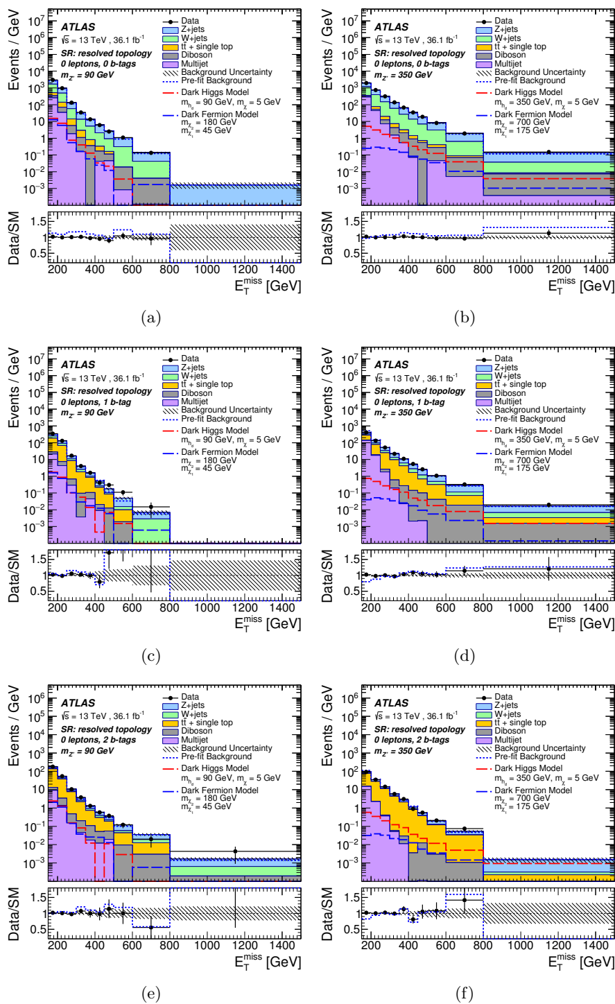
Figure 8. The observed (dots) and expected (histograms) distribution of missing transverse momentum, E_T^{\text{miss}} , obtained with 36.1 \text{ fb}^{-1} of data at \sqrt{s} = 13 TeV in the mono- Z' signal region with the resolved event topology after the profile likelihood fit (with \mu = 0 ), shown separately for the (a,b) 0b , (c,d) 1b and (e,f) 2b -tag event categories. On the left-hand side, the mediator mass of 90 GeV and on the right-hand side of 350 GeV is assumed. The total background contribution before the fit to data is shown as a dotted blue line. The hatched area represents the total background uncertainty. The expectations for the selected dark-Higgs (dashed red line) and dark-fermion (dashed blue line) signal points are shown for comparison. The inset at the bottom of each plot shows the ratio of the data to the total post-fit (dots) and pre-fit (dotted blue line) background expectation.
