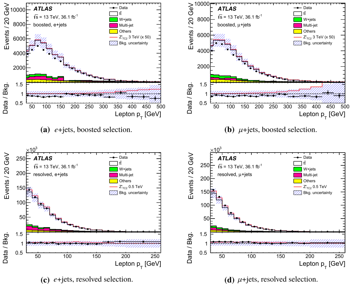
Fig. 4 The distribution of the transverse momentum of the lepton in the a boosted e+jets , b boosted \mu+jets , c resolved e+jets , and d resolved \mu+jets selections. The SM background components are shown
