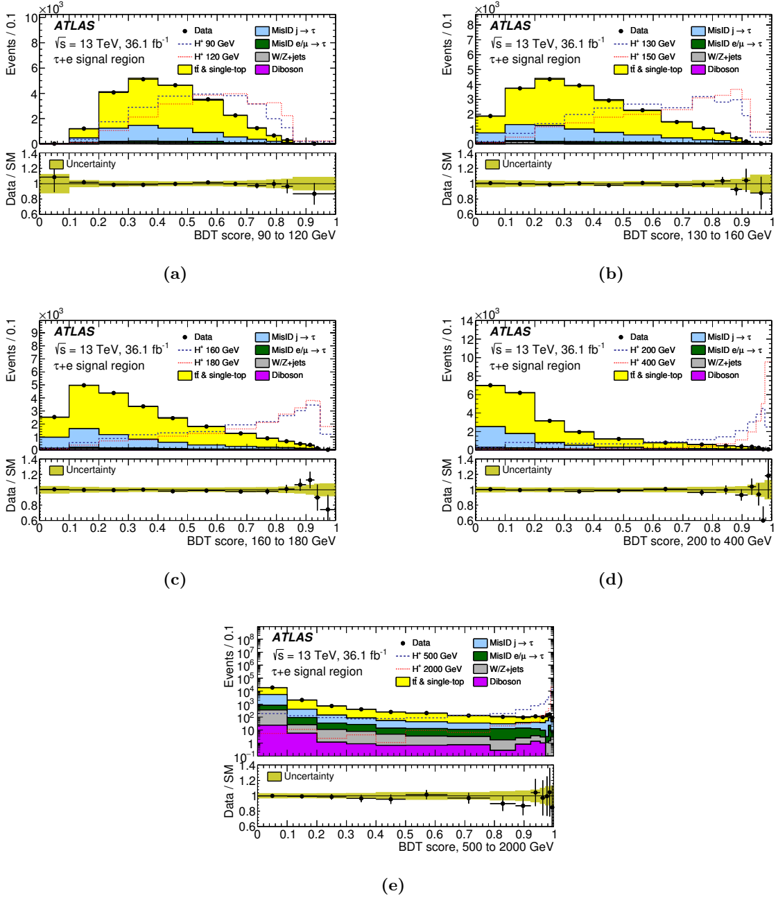
Figure 6. BDT score distributions in the signal region of the \tau_{\text{had-vis}} + \text{electron} sub-channel, in the five mass ranges used for the BDT trainings, after a fit to the data with the background-only hypothesis. The lower panel of each plot shows the ratio of data to the SM background prediction. The uncertainty bands include all statistical and systematic uncertainties. The normalisation of the signal (shown for illustration) corresponds to the integral of the background.
