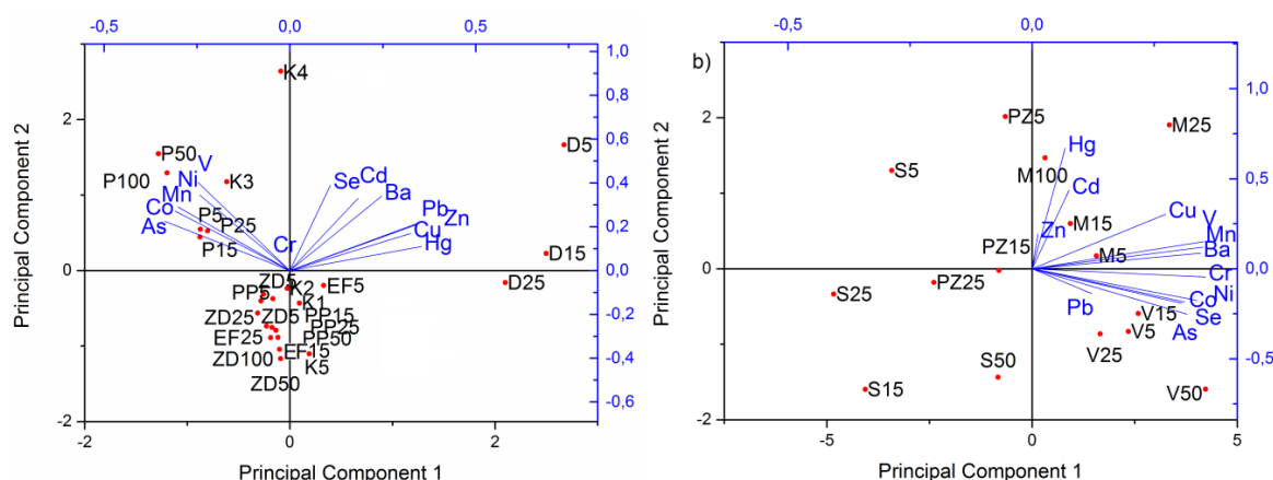
Figure 1. Principal component analysis (PCA) of extracted elements and samples within (a) industrial and (b) non-industrial areas.
