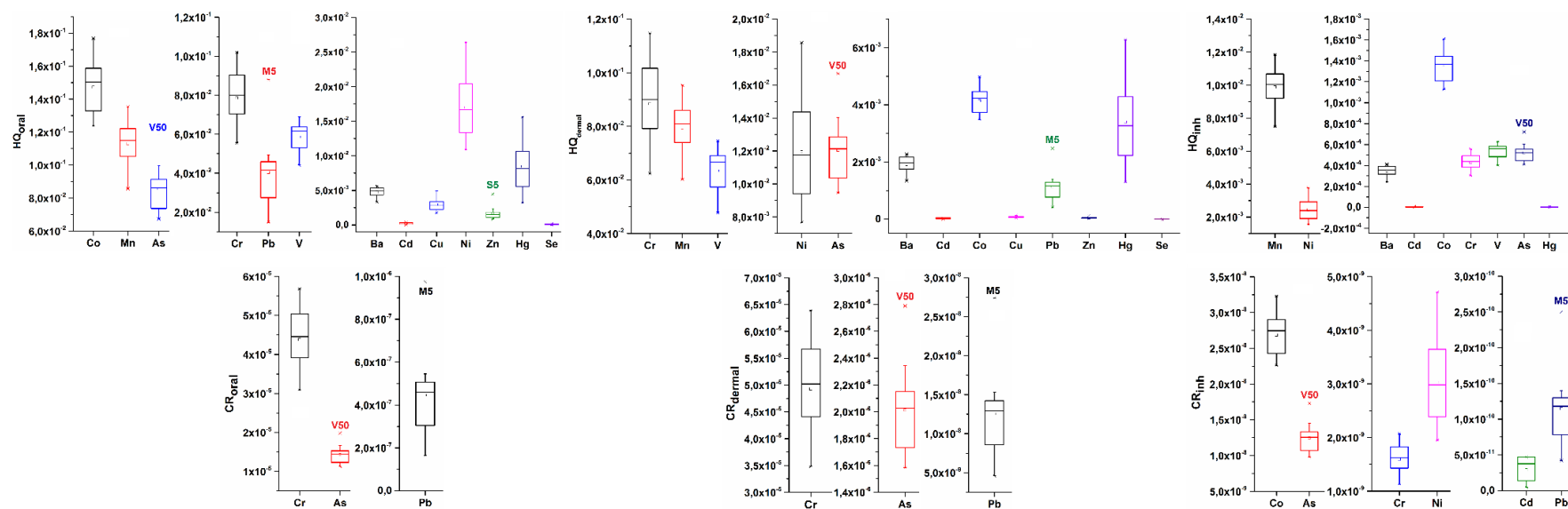
Figure 4. Hazard quotients (HQ) and cancer risk of elements for three exposure routes, oral, dermal, and inhalation (inh) in samples from the non-industrial area.
