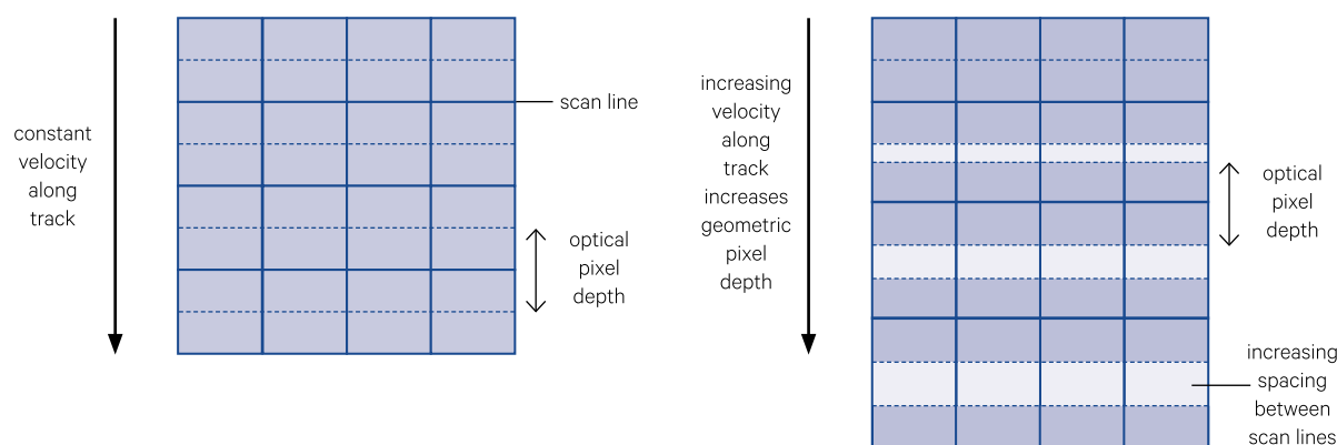
Figure 2.14 Platform velocity variation
