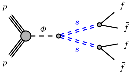
FIG. 1. Diagram for a Higgs boson or heavy scalar \Phi decaying into displaced hadronic jets via a hidden sector.
