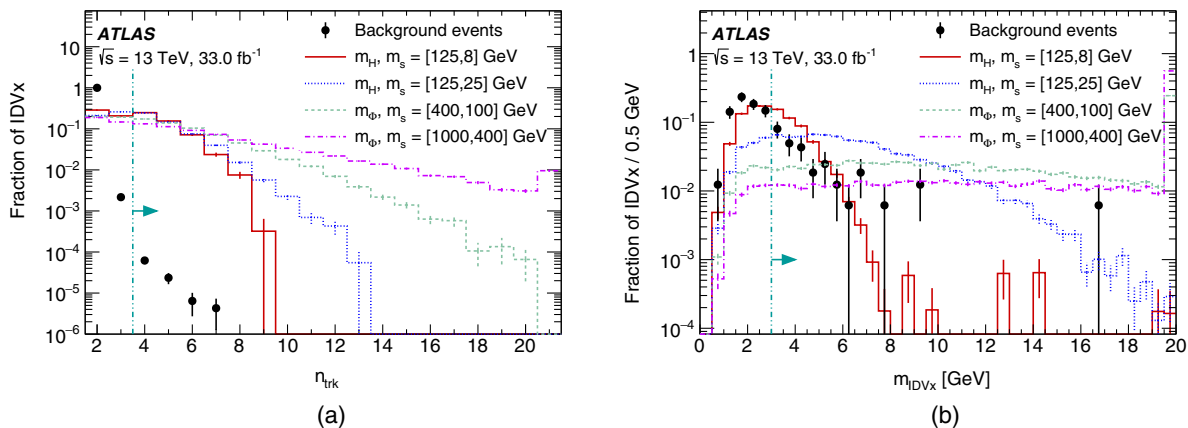
FIG. 2. Distributions of (a) n_{\text{trk}} and (b) m_{\text{IDVx}} for simulated signal MC and data background samples. The vertices shown are required to pass all selection requirements outlined in Table IV except the one displayed in the plot. The dashed lines and arrows indicate the selection requirement on the parameter shown. The last bin includes overflow.
