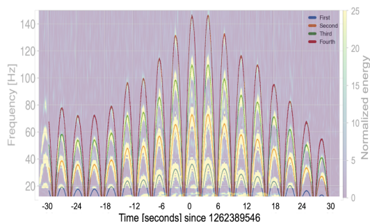
(a) PUM stage fringe frequency overlaid on h(t) scattering arches.
