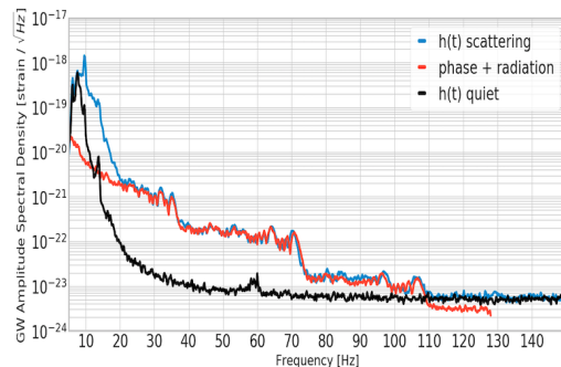
(b) PUM stage amplitude spectral density overlaid on h(t) spectrum.
