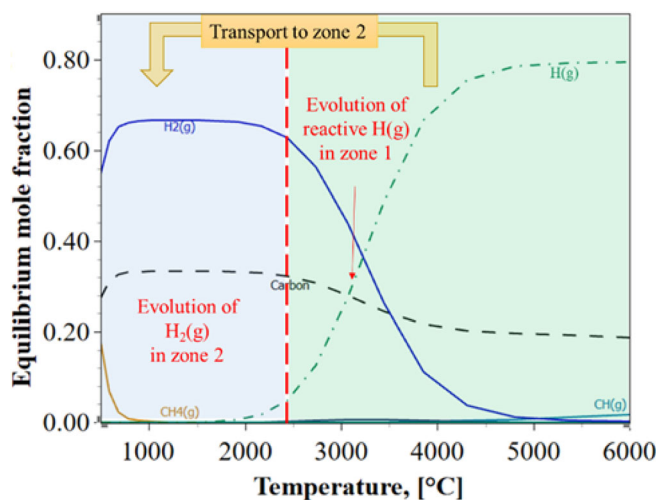
FIGURE 6 Variation of the mole fraction of the components with temperature in the thermal plasma reactor (TPR)
