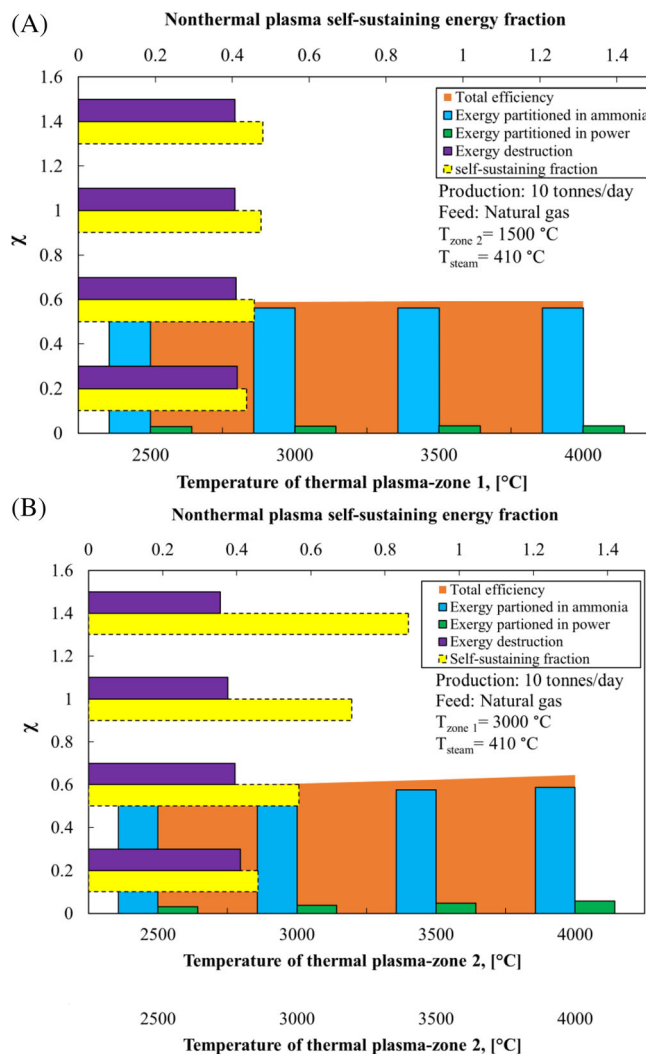
FIGURE 7 (A) Variation of the exergy partitioned in the system versus the temperature of a thermal plasma reactor in zone 1 and (B) variation of the exergy partitioned in the system versus the temperature of a thermal plasma reactor in zone 2
