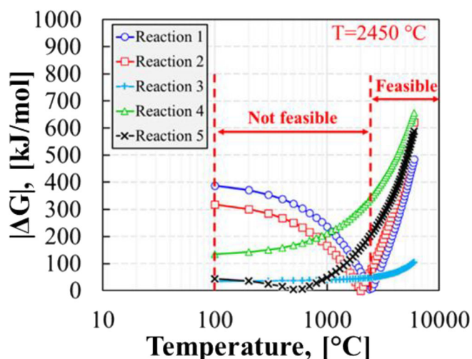
FIGURE 4 Variation of the calculated Gibbs free energy of the reactions with temperature for the one-zone thermal plasma reactor
