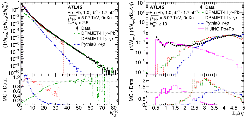
FIG. 4. Left: N_{\text{ch}}^{\text{rec}} distribution in data, corrected for trigger and reconstruction efficiency and normalized per event (black points), compared with that in DPMJET-III \gamma + Pb (dot-dashed green histogram), DPMJET-III \gamma + p (dotted red histogram), and PYTHIA \gamma + p (dashed blue histogram). The bottom panel shows the ratios of the MC distributions to the data distributions. Right: \Sigma_{\gamma} \Delta\eta distribution in data for N_{\text{ch}}^{\text{rec}} \geq 10 (black points), normalized per event, and compared with that in DPMJET-III \gamma + Pb (dot-dashed green histogram), PYTHIA \gamma + p (dashed blue histogram), peripheral HIJING Pb+Pb (solid magenta histogram), and DPMJET-III \gamma + p (dotted red histogram).
