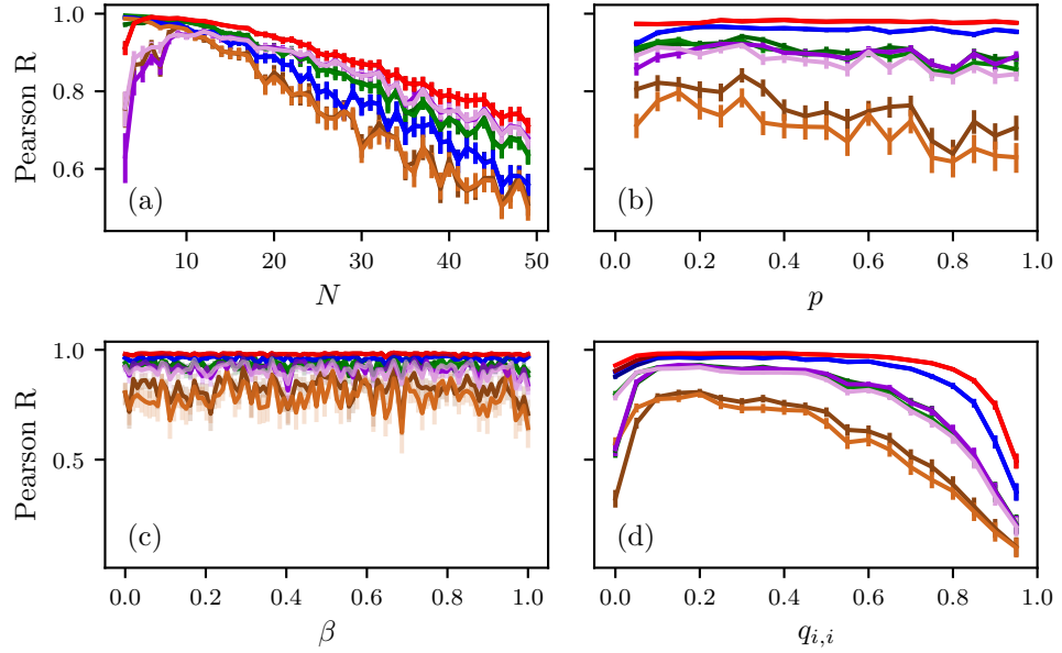
Figure 5.9: Networks are generated with N nodes where each pair of nodes has an directed edge that exists with probability p and is assigned a quote probability q'_{ji} . These quote probabilities are normalised such that their sum added to the fixed self generation probability, q_{ii} equals 1. This self generation process draws from the Twitter history of a news outlet which is assign at network creation. (b), (c) and (d) use N = 20 while (a) varies N . (a), (b) and (c) use q_{ii} = 0.5 while (d) varies q_{ii} . (a) and (d) use p = 1 while (b) varies p and (c) uses a more sophisticated Watt-Strogatz model which starts as a lattice with p = 0.4 and requires edge endpoints with probability \beta . All simulations using real data for text generation follow the same results as their counterpart experiments using Zipf distributions for text generation.
