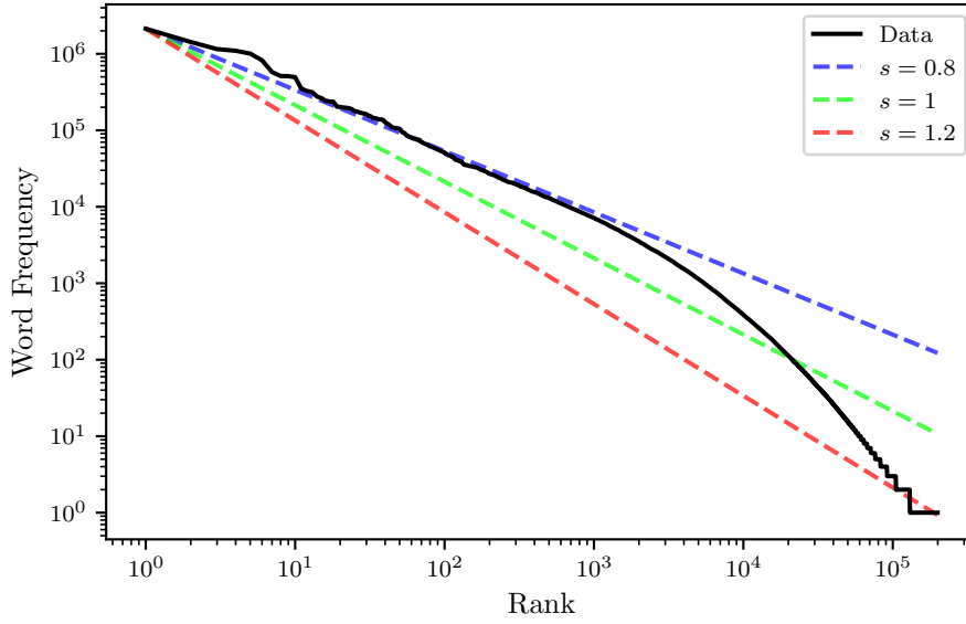
Figure 3.6: Word frequency of tokens in the corpus of all tweets produced by all news-media organisations compared the rank of the tokens by frequency. Zipf law distributions are also shown for varying scaling parameters, \alpha .
