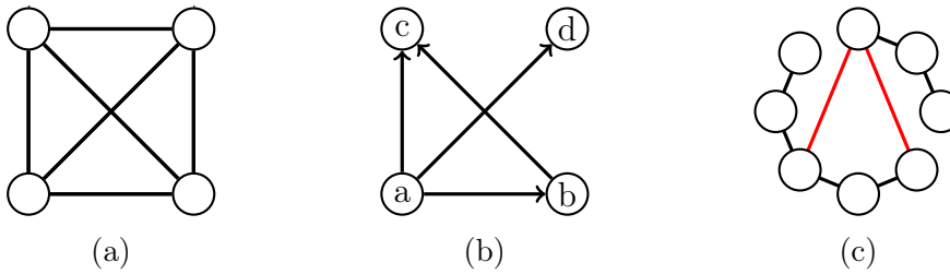
Figure 2.1: Three examples of graphs and networks. (a) is an undirected clique graph with four nodes. (b) is a directed Erdős–Rényi network with four labelled nodes and p = 2/3 . (c) is a undirected Watts-Strogatz graph with n = 8 , k = 2 and \beta = 0.25 , where rewired edges are coloured red.
