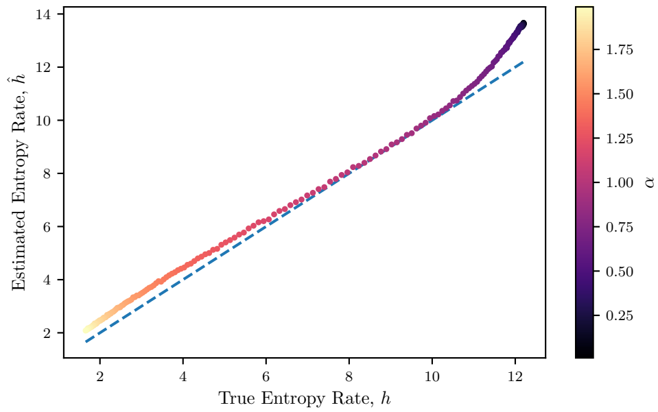
Figure 4.3: Estimated entropy rates and analytic entropy rates of sequences of 20,000 i.i.d. Zipf distribution random variables with scaling parameter \alpha . Dashed line represents the true entropy rate equalling the entropy rate estimate. As values for \alpha approach 0 the high variance of the distributions results in poor estimates due to the finite sample of the Zipf distribution.
