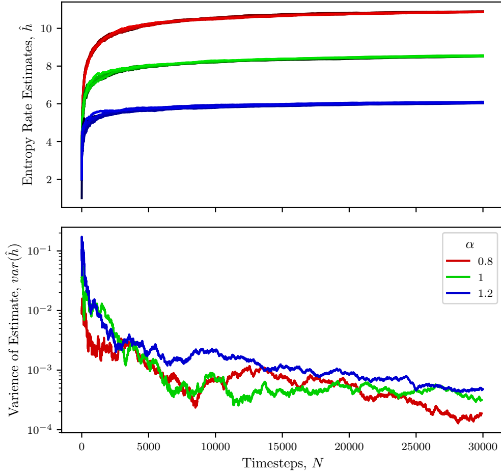
Figure 4.2: Convergence of the Kontoyiannis entropy rate estimator on sequences of i.i.d. Zipf distribution realisations with varying Zipf distribution rates, \alpha .
