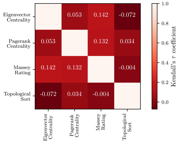
Figure 6.4: A comparison of the ordinal association between the rankings of each measure when applied to the information flow graph. All four measures show a limited correlation between each other, with the topological approach differing most from the non-negative matrix approaches.
