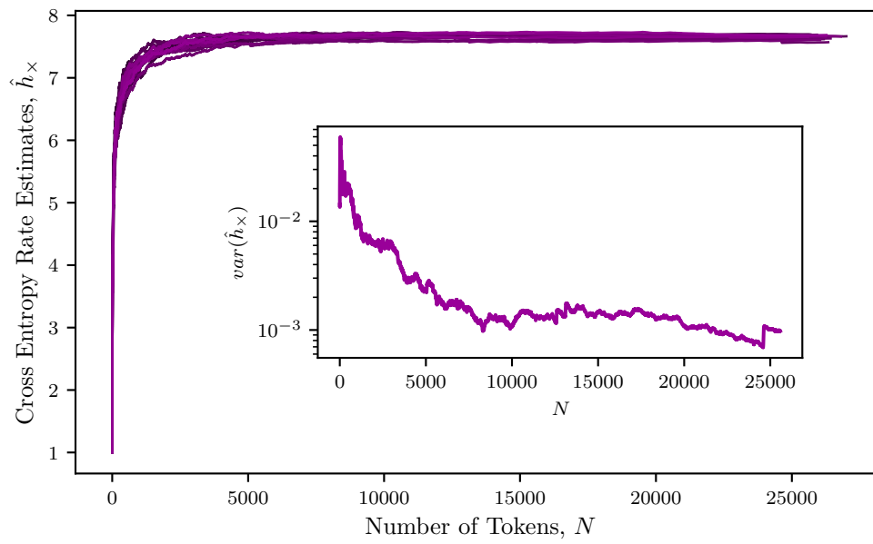
Figure 4.8: Convergence of the Kontoyiannis time-synced cross entropy rate estimator on pairs of sequences independently generated by drawing tweets uniformly without replacement from the pool of all tweets produced by all news-media organisations.
