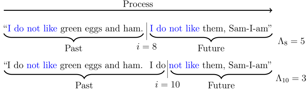
Figure 4.1: An example calculation of the match-length based \Lambda_i applied to a words in a line of text from Green Eggs and Ham by Doctor Seuss. The blue texts are words which have been matched from past to the future. As i changes, the longest match length possible starting at index i will change.
