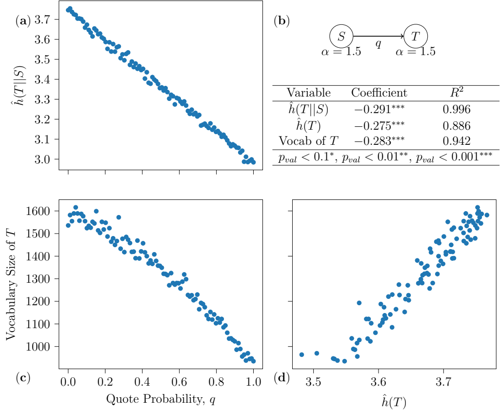
Figure 5.1: Simulations with node S generating text from a Zipf distribution with scaling parameter \alpha = 1.5 and node T generating similarly with probability 1 - q or quoting from S with probability q . While the cross entropy rate is tightly correlated with q (a), so too is the vocabulary size of T (c) and the self entropy rate of T (d). Simple linear models demonstrate that these comparison-free measures in (c) and (d) capture almost the same amount of explanatory information of q as the cross entropy.
