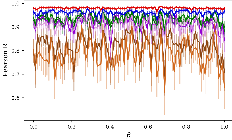
Figure 5.8: A Watts–Strogatz random graph is generated with N = 20 nodes and each edge assigned a direction and quote probability. These edges rewire with probability \beta . Information flow measures perform at consistent levels for all values of \beta , indicating that changing network structure has no impact on measure performance. High variance in correlation is seen for measure b (brown) with medium variance in d (purple) and a (green). This variance is exemplified by the large confidence intervals on the Pearson correlation coefficient which stands in contrast to the tight confidence intervals and low variance of measures e (red) and c (blue).
