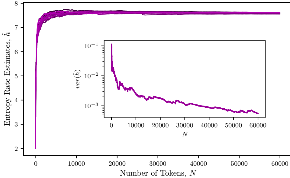
Figure 4.4: Convergence of the Kontoyiannis entropy rate estimator on sequences of words generated by drawing tweets uniformly without replacement from the pool of all tweets produced by all news-media organisations. Multiple sequences are drawn with most convergence curves overlapping.
