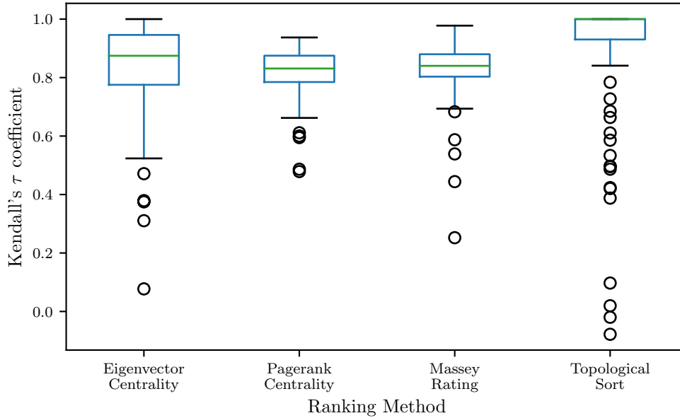
Figure 6.3: Network ranking measures undergo sensitivity testing by ranking the network with a single node removed and comparing to the original ranking. This is repeated for each possible node removal in the network for all ranking measures. All measures show an average positive correlation between new and original rankings, with a high degree of variance in the sensitivity. PageRank has the best worst-case and worst average-case while topological sorting has the best average-case and worst worst-case.
