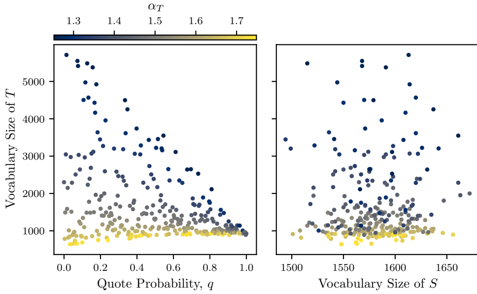
Figure 5.4: The target node T self generates with probability 1-q from a Zipf distribution according to a variable scaling parameter, \alpha_T \sim U(1.25, 1.75) . With probability q , T quotes from the source, S , which always self generates with \alpha_S = 1.5 . The added variability in the self generation at T decouples the previous tight correlation between the vocabulary size and the self generation probability.
