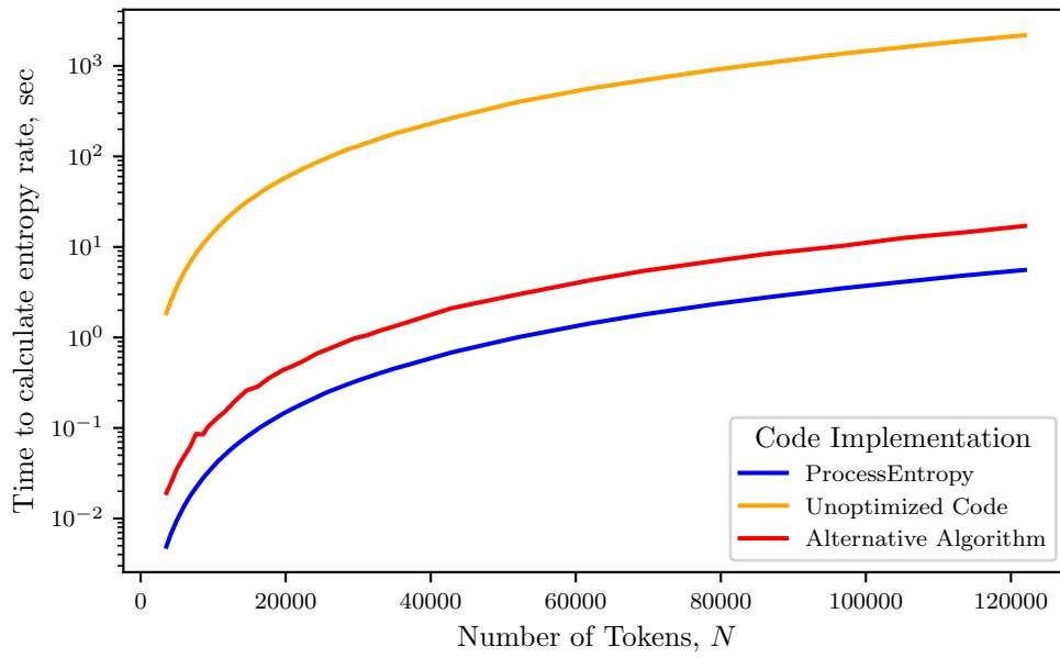
Figure 4.10: A speed comparison of implementations of the Kontoyiannis entropy rate estimator. ProcessEntropy uses code from the package of the same name, unoptimized code is the same algorithm as ProcessEntropy without type and compile optimizations and Alternative Algorithm is an optimized alternative algorithm using the built-in .contains() method from the stringlib library.
