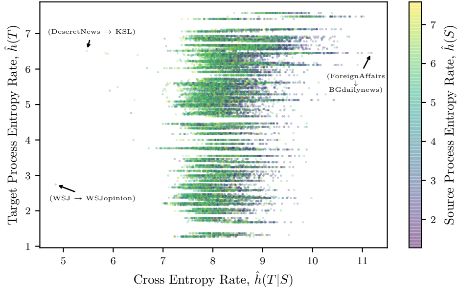
Figure 4.12: Time-synced cross entropy rate estimates on pairs of news-media organisations on Twitter using their full content for the 2019 calendar year. Cross entropy rates are compared to the entropy rate estimates of the sources, S , and targets, T , in isolation. Example outliers are shown as ‘(source → target)’.
