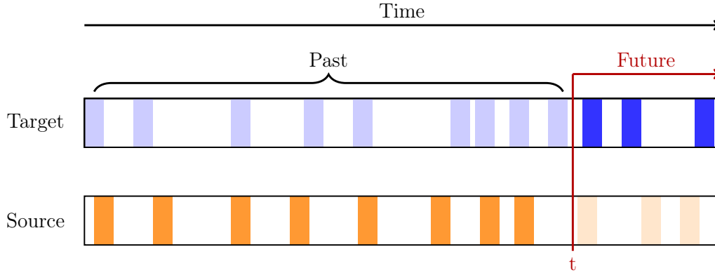
Figure 4.7: A conceptual diagram of Kontoyiannis time-synced cross entropy rate estimation. Tweets shown as rectangles are positioned in time for both a target and source, containing textual information. Content in the source that occurs before time t is matched with content in the immediate future of the target from t to calculate match-lengths. This time point is shifted along the target timeline to average match-lengths and calculate the time-synced cross entropy rate.
