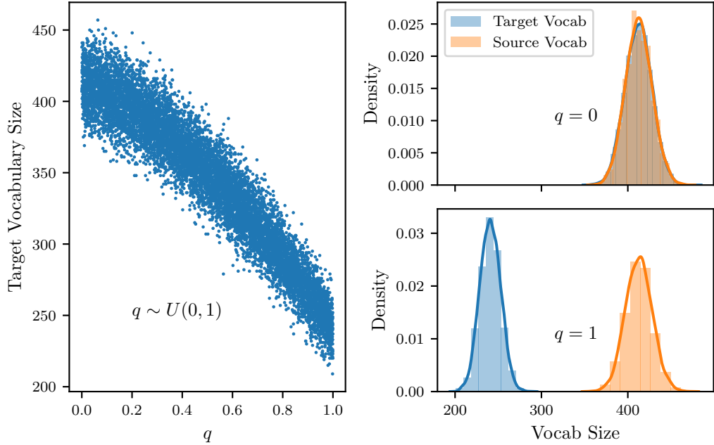
Figure 5.2: A source produces text from a Zipf distribution of words. A target produces text similarly with probability 1 - q or quotes from the source with probability q . The vocabulary size of the source and target are calculated by taking the number of unique elements after 1000 time steps. The vocabulary size of the target decreases as q increases.
