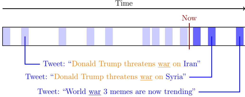
Figure 4.5: A conceptual diagram of entropy rate estimation using the Kontoyiannis entropy rate estimation. Tweets shown as blue rectangles are positioned in time and contain textual content. Content proceeding the position Now will have snippets of text matched with text from the history of the process, denoted by orange and underlined text. These text matches are used to calculate \Lambda_i which is used in the entropy estimate.
