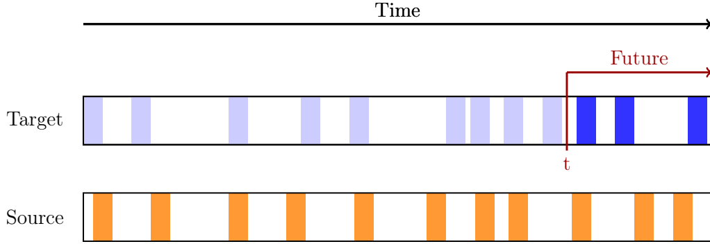
Figure 4.6: A conceptual diagram of Kontoyiannis full cross entropy rate estimation. Tweets shown as rectangles are positioned in time for both a target and source, containing textual information. Content in the source is matched with content in the immediate future of the target for a given time point, t , to calculate match-lengths. This time point is shifted along the target timeline to average match-lengths and calculate the full cross entropy rate.
