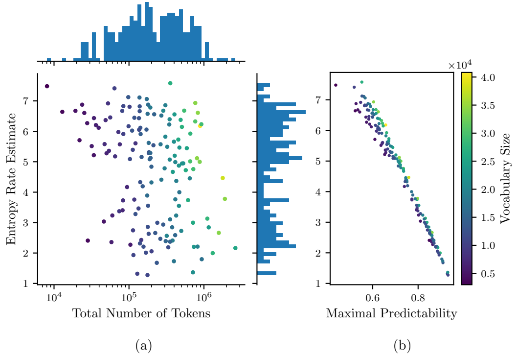
Figure 4.11: Entropy rate estimates for the Twitter timelines of 154 news-media organisations during the calendar year of 2019. (a) shows the limited relationship between the total number of tokens in the Twitter text history and the entropy rate estimates. (b) shows the tight relationship between the entropy rates estimate and its derived maximal predictability, with higher variances seen at high entropies.
