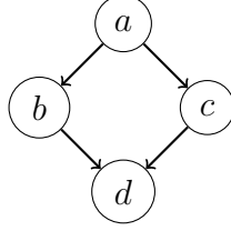
Figure 6.2: A demonstration of the diamond problem that can give non-unique solutions to naive topological sorts on directed acyclic graphs.
