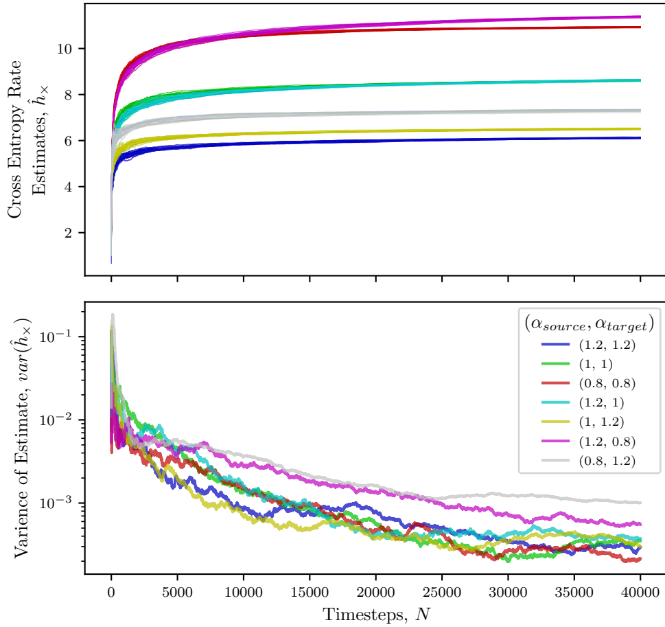
Figure 4.9: Convergence of the Kontoyiannis time-synced cross entropy rate estimator on pairs sequences of i.i.d. Zipf distribution realisations with varying pairs of Zipf distribution rates, \alpha_{source} and \alpha_{target} .
