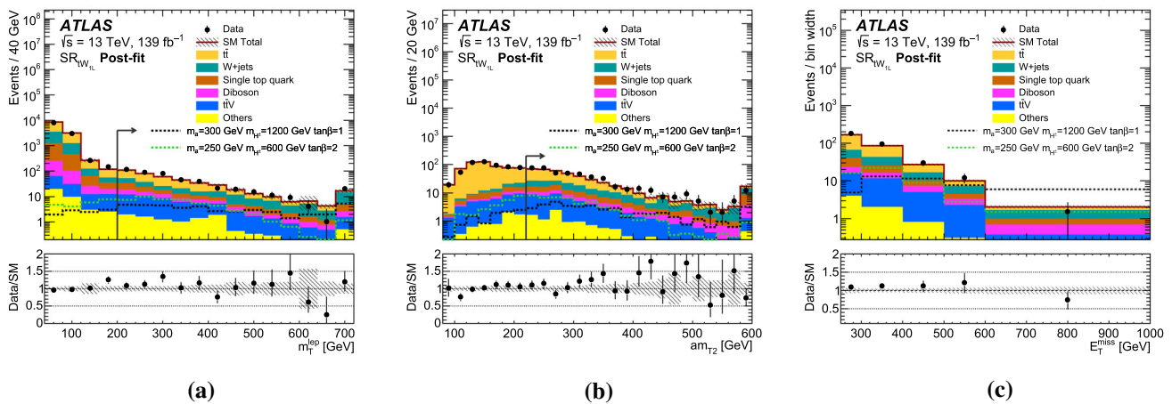
Fig. 10 Representative distributions of a m_T^{\text{lep}} , b am_{T2} and c E_T^{\text{miss}} in the tW_{1L} channel. Observed data are compared with the SM background predictions extrapolated from the background-only fit. All SR selections except the one on the quantity shown are applied. The SR requirement is indicated by the arrow. The ‘Others’ category includes contributions from Z+jets and tWZ production, and rare processes such as triboson, t\bar{t}t\bar{t} , t\bar{t}WW , and Higgs boson production processes. The expected
