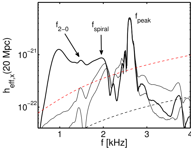
Fig. 3 Typical GW spectrum of the cross polarization of a 1.35\text{--}1.35 M_{\odot} merger along the polar direction at a distance of 20 Mpc. h_{\text{eff},x} = \tilde{h}_x(f) \cdot f with the Fourier transform of the waveform h_x and frequency f . f_{\text{peak}} , f_{\text{spiral}} and f_{2-0} are particular features of the post-merger phase, which can be associated with certain dynamical effects in the remnant. Since the simulation started only a few orbits before merging, i.e. at a relatively high orbital frequency, the power at lower frequencies (below \sim 1 kHz) is massively under-represented in the shown spectrum, and the low-frequency part of the spectrum does not show the theoretically expected power-law decay. The thin solid lines display the spectra of the GW signal of the post-merger phase only revealing that the peaks are indeed generated in the post-merger phase. Dashed lines show the expected unity signal-to-noise sensitivity curves of Advanced LIGO (red) and of the Einstein Telescope (black). Image reproduced with permission from Bauswein et al. (2016), copyright by SIF/Springer
