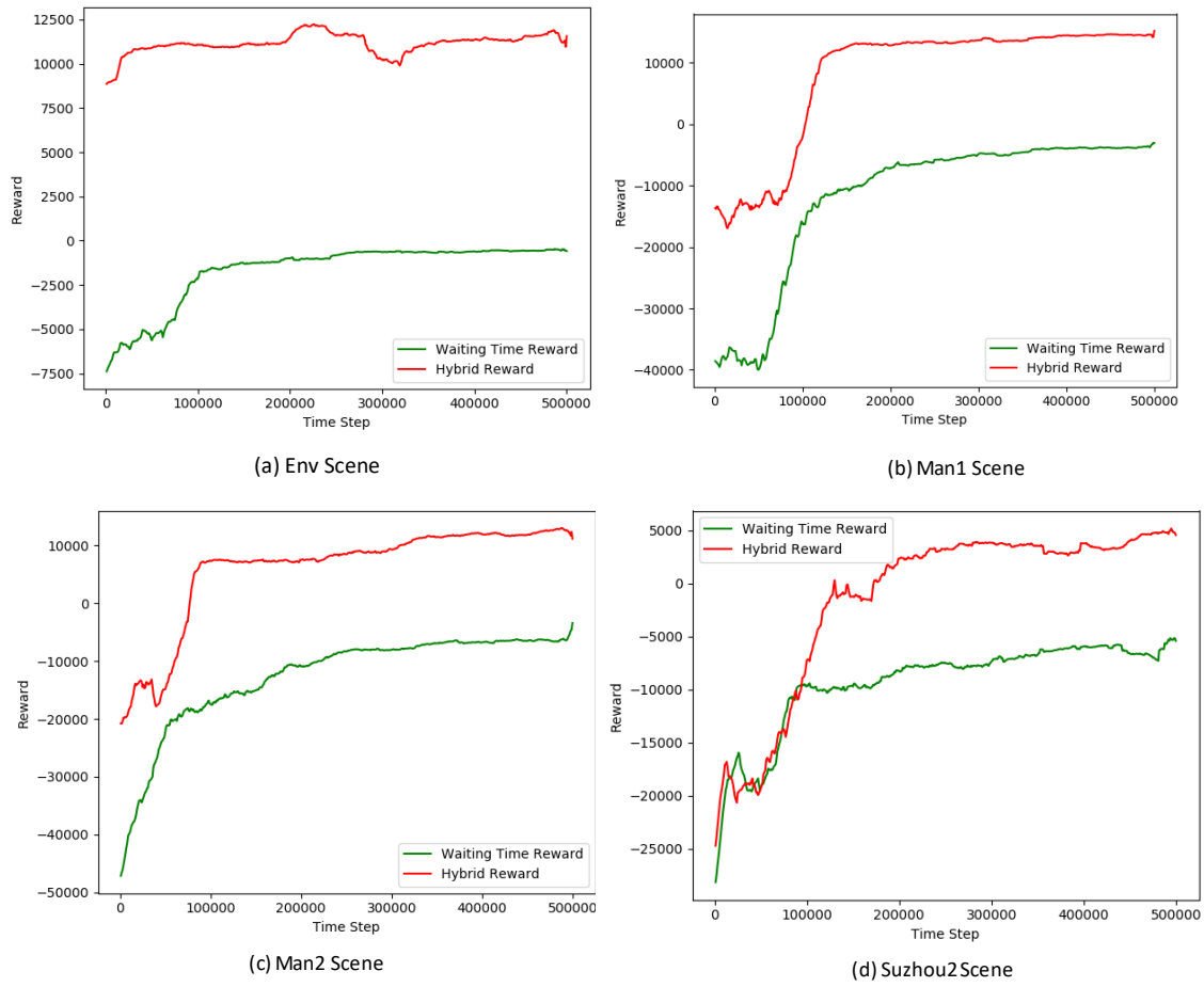
FIGURE 3.10. Comparison of EGU-RL with hybrid reward and with only waiting time reward under different scenes. The proposed algorithm can obtain higher reward with hybrid reward, which suggests the effectiveness of hybrid reward to practically control the frequency of traffic signals.
