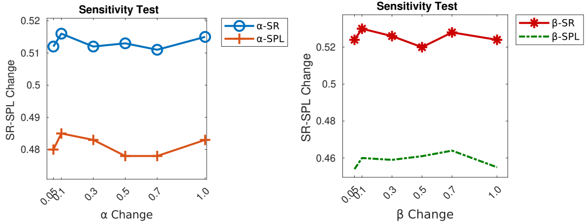
FIGURE 4.4. The sensitivity test of our Soft Expert Reward Learning (SERL) model. The figures show the SR and SPL performance of the model on validation unseen set with different \alpha and \beta values.
