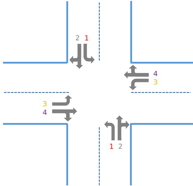
FIGURE 3.1. An example of traffic signals (right-side driving). As shown in the figure, the numbers represent different phases. In each round, phases are switched from “1” to “4” sequentially to allow different traffic streams to pass the junction without collision.
