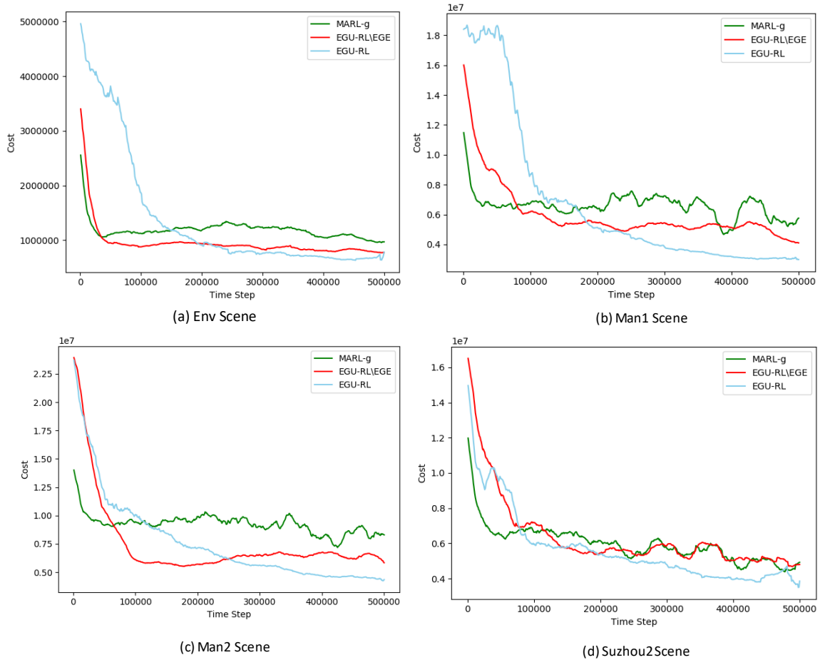
FIGURE 3.8. Convergence comparison of different models on total accumulative waiting time cost (the lower the better) under different scenes. The EGU-RL algorithm surpasses MARL-g and w/o EGE algorithms and achieved the lowest accumulative waiting time costs in the end.
