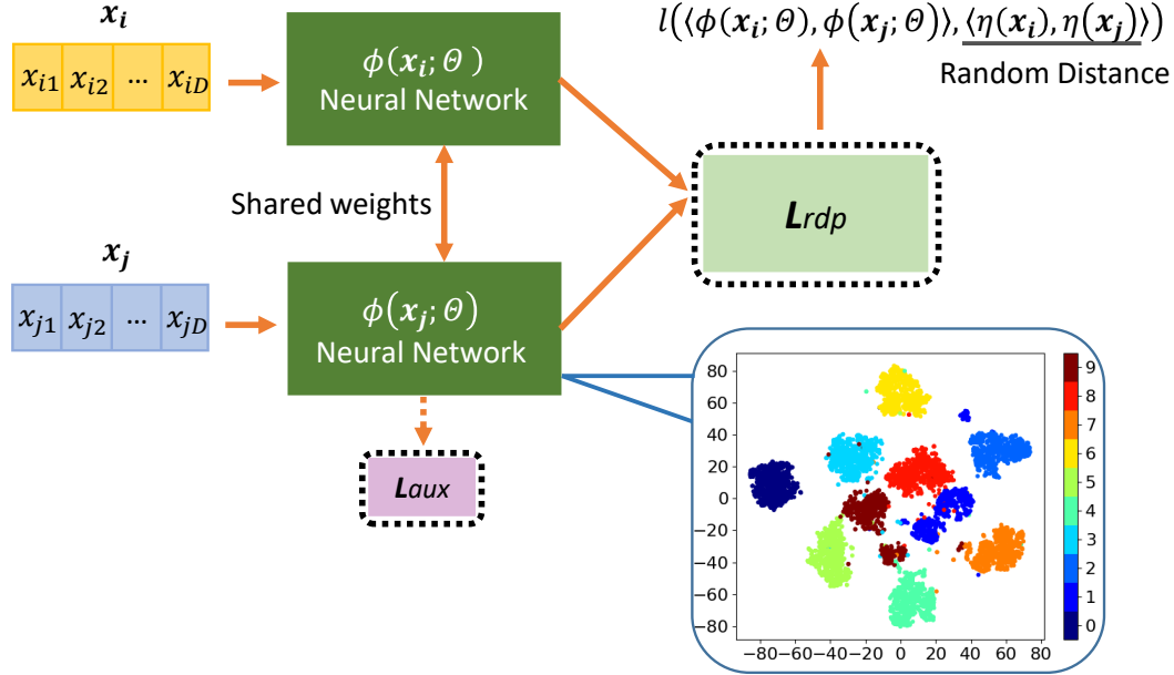
FIGURE 5.1. The proposed random distance prediction (RDP) framework. Specifically, a weight-shared two-branch neural network \phi first projects \mathbf{x}_i and \mathbf{x}_j onto a new space, in which we aim to minimise the random distance prediction loss L_{rdp} , i.e., the difference between the learned distance \langle \phi(\mathbf{x}_i; \Theta), \phi(\mathbf{x}_j; \Theta) \rangle and a predefined distance \langle \eta(\mathbf{x}_i), \eta(\mathbf{x}_j) \rangle ( \eta denotes an existing random mapping). L_{aux} is an auxiliary loss that is optionally applied to one network branch to learn complementary information w.r.t. L_{rdp} . The lower right figure presents a 2-D t-SNE (Hinton and Roweis, 2003) visualisation of the features learned by RDP on a small toy dataset optdigits with 10 classes.
