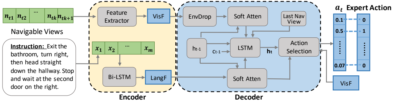
FIGURE 4.2. Encoder-Decoder Structure of Soft Expert Reward Learning (SERL) framework. After fetching the visual and language features from the encoder, the multi-modal features are fed into the decoder to obtain cross-modal attentions. Finally, actions will be chosen according to the attentive features.
