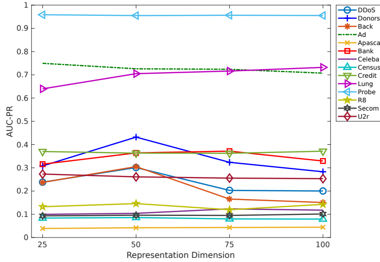
FIGURE 5.3. AUC-PR results of RDP w.r.t. different representation dimensions on 14 datasets.
