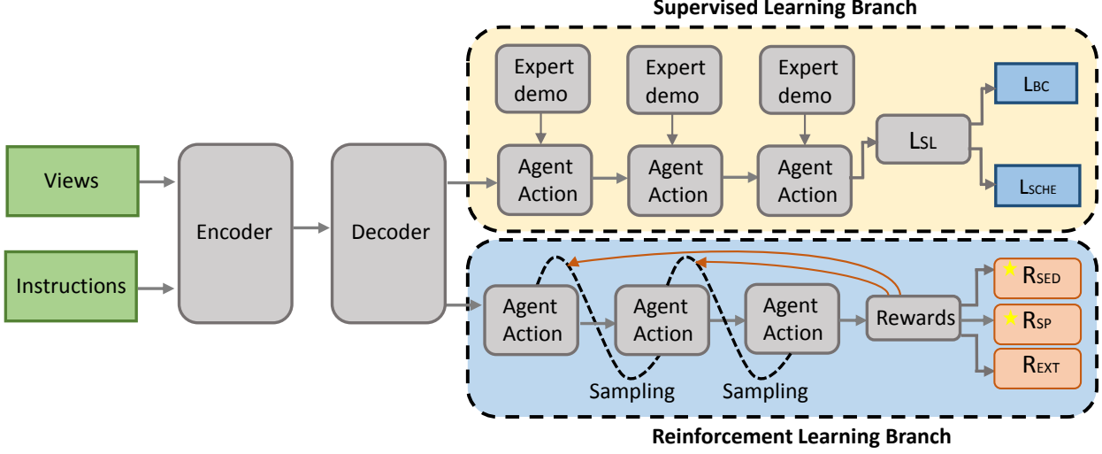
FIGURE 4.1. The proposed Soft Expert Reward Learning (SERL) framework. After getting the visual features and language features through the encoder, they are fed into the decoder to obtain the selected action a_t for time step t . The training process of SERL is divided into two parts: a supervised learning branch and a reinforcement learning branch. We introduce two novel rewards (marked with yellow stars in the figure): Soft Expert Distillation (SED) reward and Self Perceiving (SP) reward.
