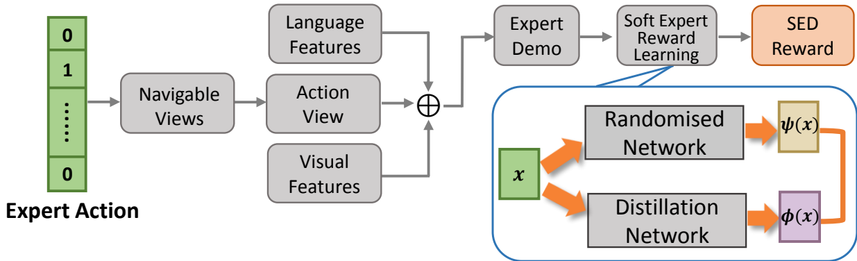
FIGURE 4.3. The Soft Expert Distillation networks structure. Given an expert demonstrated data point x \in \mathbb{R}^N , it is fed into a weight-fixed randomly initialised neural network \psi(\mathbf{x}) ; simultaneously, the data point x is inputted into a distillation network \phi(\mathbf{x}; \theta) with different structure but same output dimensions with the parameters \theta .
