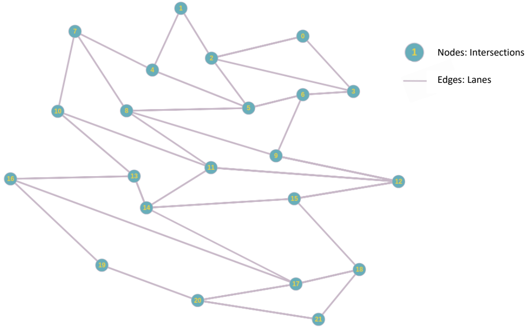
FIGURE 3.5. An Instance of graph model, which can be processed by Graph Convolutional Networks, to represent Junctions of several blocks in Manhattan. Each node represents an intersection and each edge represents a lane connection between two nodes.
