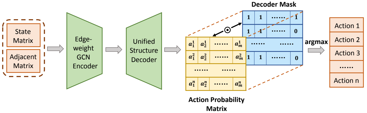
FIGURE 3.4. The proposed EGU-RL Model. The figure represents our proposed EGU-RL model with the Edge-weighted Graph Convolutional Encoder and the Unified Structure Decoder.
