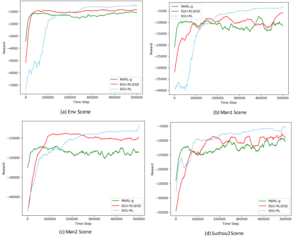
FIGURE 3.9. Convergence comparison of different models on total rewards (the higher the better) under different scenes. EGU-RL algorithm surpasses MARL-g and w/o EGE algorithms and gets the highest reward in the end.
