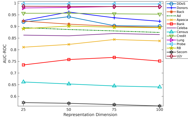
FIGURE 5.2. AUC-ROC results of RDP w.r.t. different representation dimensions on 14 datasets.
