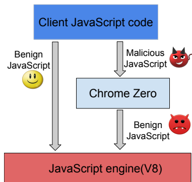
Figure 6: High-level concept of Chrome Zero
