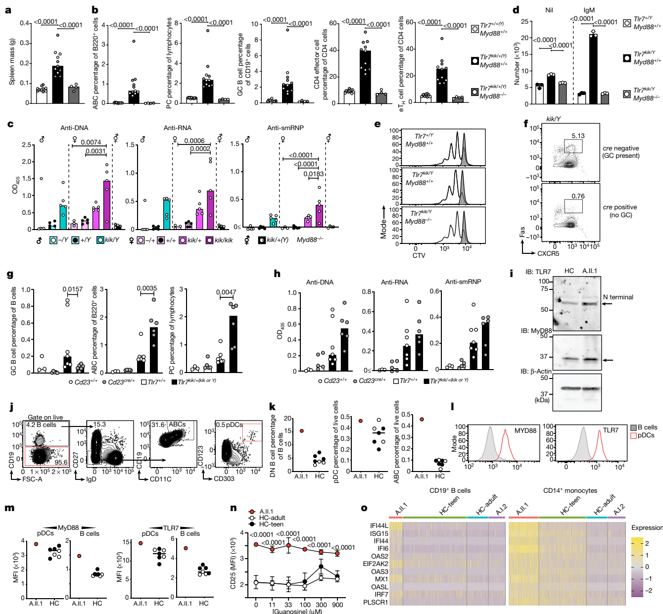
Fig. 4 | TLR7-mediated autoimmunity is MyD88 dependent. a, b , Spleen mass ( a ) and flow cytometry quantification ( b ) of ABCs (B220 + CD21 + CXCR5 + CD19 high CD11c + ), plasma cells (CD138 + CD98 + ), GC B cells (CD19 + CD95 + BCL6 + ), CD4 effector/memory T cells (CD4 + FOXP3 + CD44 + ) and extrafollicular helper cells (CD4 + CXCR5 + PD1 + CXCR3 + ) from splenocytes of male (grey) and female (white) kika mice (aged 12 weeks) either sufficient or deficient in MyD88. c , Auto-antibodies to ssDNA (ANAs), ssRNA and smRNP from kika mice (aged 12 weeks) either deficient or sufficient in MyD88. d, e , Survival ( d ) and proliferation ( e ) of CTV-labelled splenic B cells cultured for 72 h with anti-IgM (white) or unstimulated (grey). f, g , Flow cytometry plots ( f ) and quantification ( g ) of splenic GC B cells (CD19 + CD95 + CXCR5 + ), ABCs and plasma cells from kika or control littermates (aged 10 weeks) either deficient ( Bcl6 fllox/fllox ; Cd23 cre ) or sufficient ( Bcl6 fllox/fllox ) in GCs ( Cd23 +/+ n = 3, Cd23 cre/+ n = 5, Tlr7 +/+ n = 7, Tlr7 kik/+ (kik or Y) n = 6). h , Serum autoantibodies to ssDNA, ssRNA and smRNP in the same mice as in g . i , Western blots showing TLR7 and MyD88 expression in PBMCs from A.II.1 and an age- and gender-matched healthy control individual (HC). j, k, l , Flow
