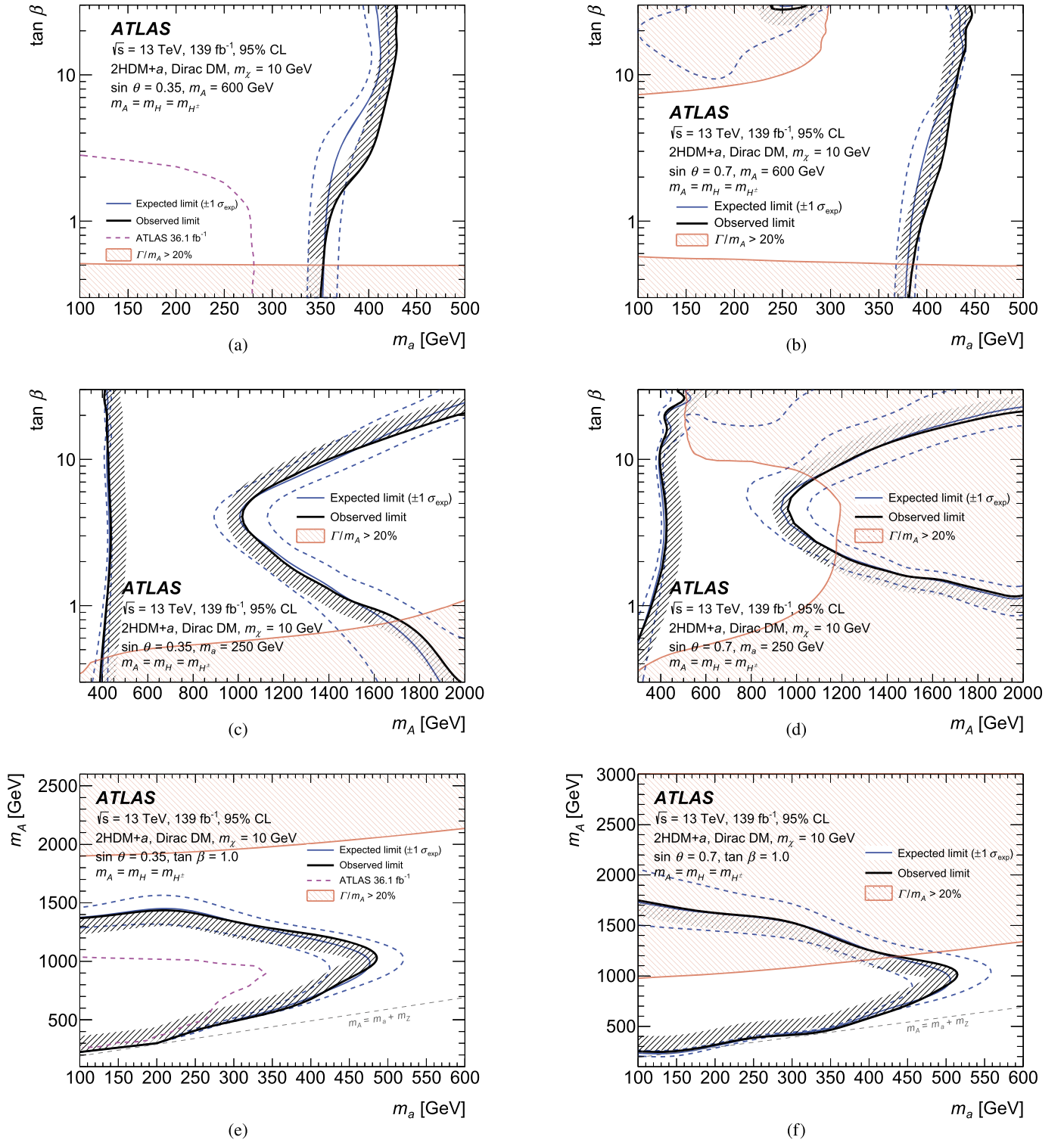
Fig. 5. Exclusion limits within the context of 2HDM+a models with different parameter choices and in various planes [17]. Subfigures (a, b) show the \tan\beta vs m_a exclusion limits with m_A = 600 GeV, (c, d) the \tan\beta vs m_A exclusion limits with m_a = 250 GeV, and (e, f) the m_A vs m_a exclusion limit with \tan\beta = 1.0 . The region contained by the solid black line and the hashed black contour is excluded at the 95% CL. The solid blue line indicates the expected limit in the absence of signal, and the dashed blue lines the corresponding \pm 1\sigma uncertainty band. Subfigures (a, c, e) assume \sin\theta = 0.35 , while (b, d, f) assume \sin\theta = 0.7 . Where included, the dashed magenta lines represent the 36.1 \text{ fb}^{-1} results from Ref. [18]. The hashed red area indicates that the width of one of the Higgs bosons is larger than 20% of its mass.
