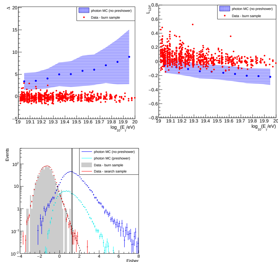
Figure 5. (Top) distributions of \Delta (left) and L_{\text{LDF}} (right), i.e., the observables used in the search for photons based on SD-only data, as a function of the photon energy E_\gamma for simulated primary photons (in blue) and a fraction of the data sample (in red) that is used as a burnt sample; the bands represent one standard deviation of the photon distributions. (Bottom) distributions of the Fisher discriminant for the burnt sample (grey), the search sample (red) and simulated primary photons (non-preshowering in blue and preshowering in light blue), weighted with an E^{-2} spectrum; the search sample and the photon distributions are scaled to have the same integral as the burn sample one; the vertical line indicates the value of the photon-candidate cut; the dashed line shows the result of the fit of an exponential to the 5% of events in the burnt sample with the largest values of the Fisher discriminant. For more details, see [25].
