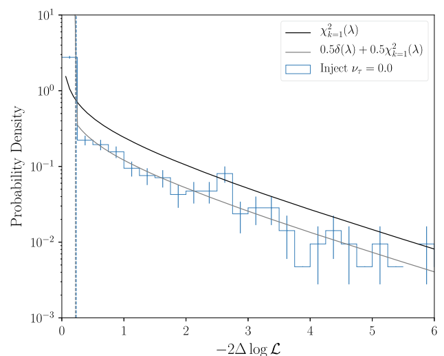
Fig. 8 Test statistic distribution of the one-dimensional pseudo Monte Carlo trials for an injected vanishing astrophysical tau neutrino flux. The expected half- \chi^2_{k=1} distribution (gray line) is followed. The \chi^2_{k=1} distribution is shown for reference (black line). The vertical lines that mark the events contributing to the 68% confidence interval (blue), and the expectation from the half- \chi^2_{k=1} distribution (gray) are almost perfectly aligned
