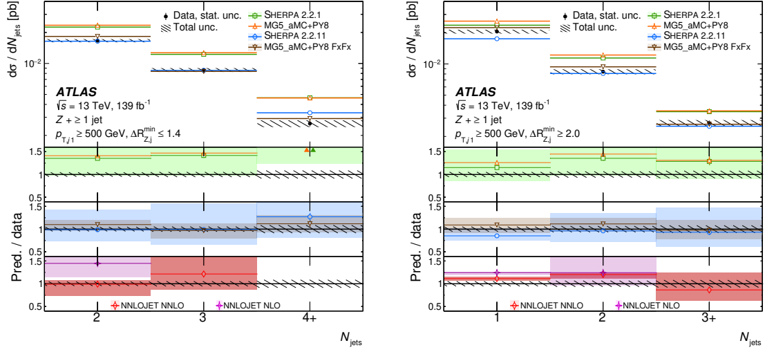
Figure 9. Differential cross section as a function of the jet multiplicity in the collinear \Delta R_{Z,j}^{\min} \leq 1.4 region (left) and in the back-to-back \Delta R_{Z,j}^{\min} \geq 2.0 region (right). In each case, the last bin is inclusive in higher jet multiplicities. In data, no events with exactly one jet are selected in the collinear region. Further details are provided in the caption of figure 5.
