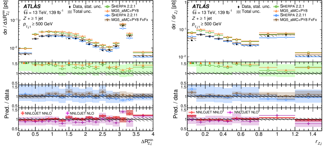
Figure 7. Differential cross section as a function of angular distance between the Z boson and the closest jet, \Delta R_{Z,j}^{\min} (left) and of the ratio of Z -boson to closest-jet transverse momenta r_{Z,j} (right) in the high- p_T region. For the NNLOJET predictions, the bins around r_{Z,j} = 1 are merged to be insensitive to the singularity in the fixed-order calculation. Further details are provided in the caption of figure 5.
