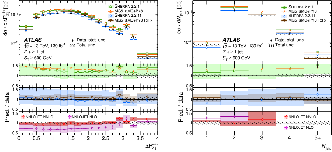
Figure 11. Differential cross section as a function of the angular distance \Delta R_{Z,j}^{\min} between the Z boson and the closest jet (left) and of the jet multiplicity (right) in the high- S_T region. In the jet-multiplicity distribution, the last bin is inclusive in higher jet multiplicities. Further details are provided in the caption of figure 5.
