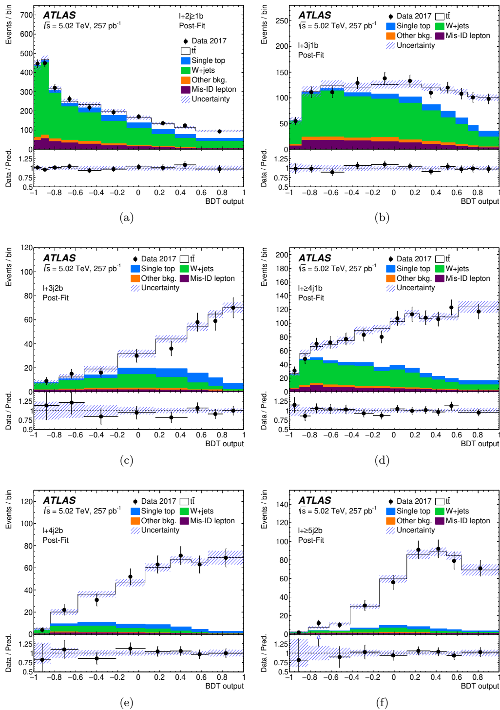
Figure 7. Comparison between data and the results of the fit to the BDT output distributions in the (a) l+2j \geq 1b region, (b) l+3j 1b region, (c) l+3j 2b region, (d) l+ \geq 4j 1b region, (e) l+4j 2b region, and (f) l+ \geq 5j 2b region. The ‘Other bkg.’ includes Z +jets and diboson backgrounds. The bottom panel displays the ratio of data to the total prediction. The hashed area represents the total uncertainty of the background.
