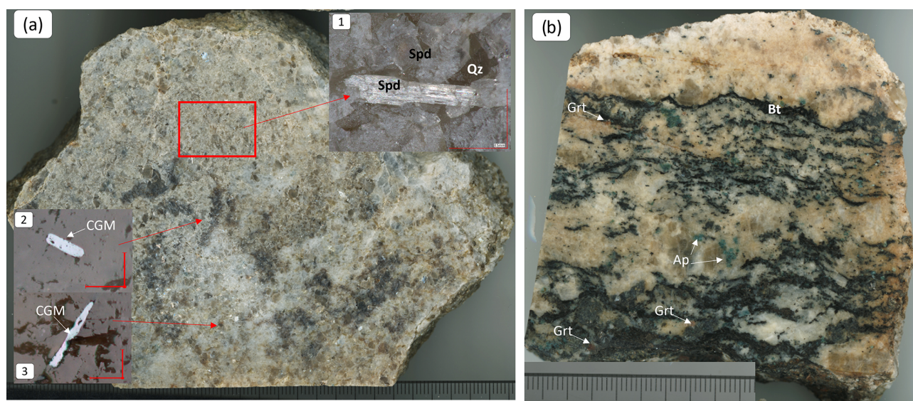
Figure 4. (a) Example of massive and fine-grained spodumene mineralisation of the main dyke. White spodumene (inset 1) occurs in 1–3 mm subhedral-to-euhedral prismatic crystals intergrown with quartz, albite, K-feldspar, and muscovite. Microscopic platelets of columbite–tantalite-group minerals (CGMs) are disseminated through the groundmass as 100–400 µm sized laths (inset 2, 3). (b) Banded albite pegmatite of the SE dyke swarm consists of distinct undulating thin layers of biotite–apatite–garnet, with quartz–albite–green apatite.
