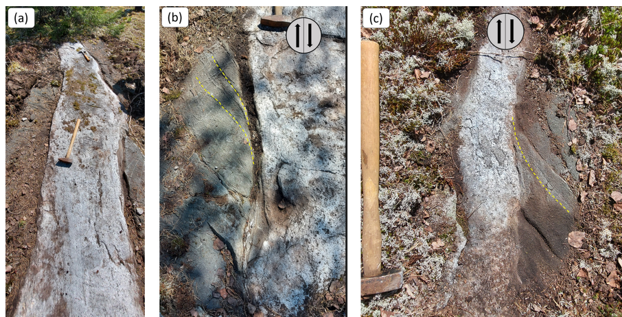
Figure 9. (a) Example of a smaller dyke in the SE dyke swarm albite pegmatite. Weak-to-moderate magmatic flow banding can be observed. (b) Deflection of the near-vertical foliation plane (shown by dashed yellow lines) in the metavolcanic bedrock along a 1 m wide dyke contact. (c) Deflection of the foliation along a 20 cm wide dyke contact. The clockwise rotation of the foliation plane suggests a dextral shear sense of the ENE-trending shear zones along which the Kietyönmäki pegmatite dykes were emplaced.
