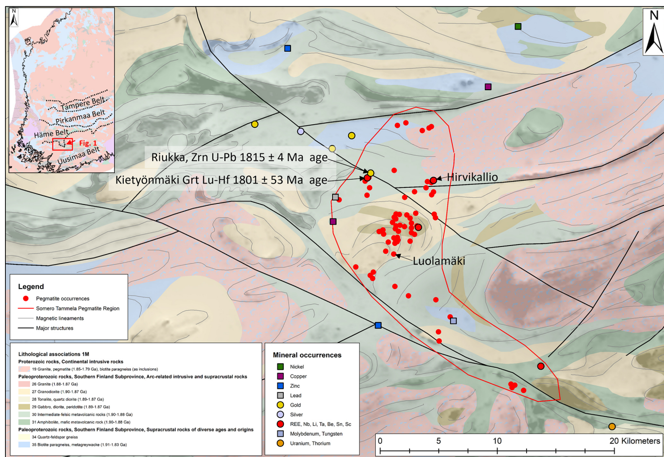
Figure 1. Regional geology map of the Somero–Tammela pegmatite region. Data source: “Bedrock of Finland” – DigiKP, digital map database, 1 : 200 000, Geological Survey of Finland, https://gtkdata.gtk.fi/mdae/index.html (last access: 21 May 2024).
