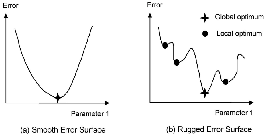
Fig. 10. Error surface with different degrees of ruggedness for a model with one parameter.
