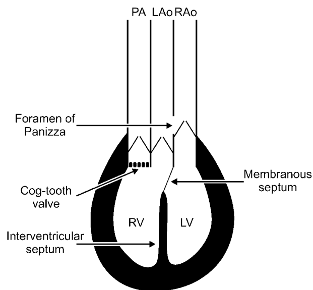
Figure 5. Schematic of the crocodilian heart, with ventricles completely separated by the interventricular and membranous septa. The foramen of Panizza connects the left and right aortic arches (LAo and RAo, respectively), and a cog-tooth valve lies beneath leaf valves in the pulmonary artery (PA).
