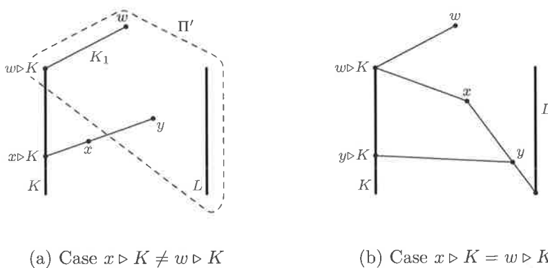
Figure 1.2: Diagrams for proof of Lemma 1.10.
