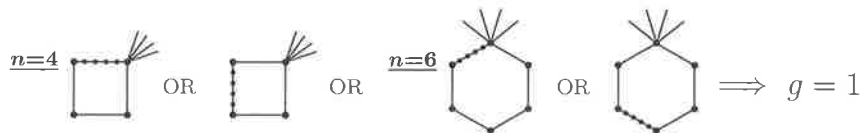
Figure 1.1: A collineation fixing so much must be the identity (Lemma 1.7).
