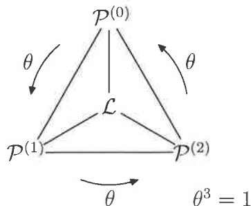
Figure 1.3: The triality \theta
