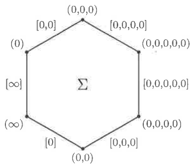
Figure 1.4: Labelling the hat-rack
