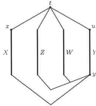
Figure 3.4: This configuration does not occur (Lemma 3.17).
