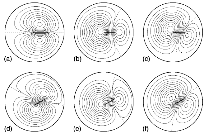
FIG. 5. Streamlines for a paddle of length 0.4, centered z=0.2+0.0i . Top row: \theta_1=0 . Translation (a) in the x -direction, (b) in the y -direction, (c) at a 45^\circ angle. Bottom row: \theta_1=\pi/6 . Translation (d) in the x -direction, (e) in the y -direction, (f) at a 45^\circ angle.
