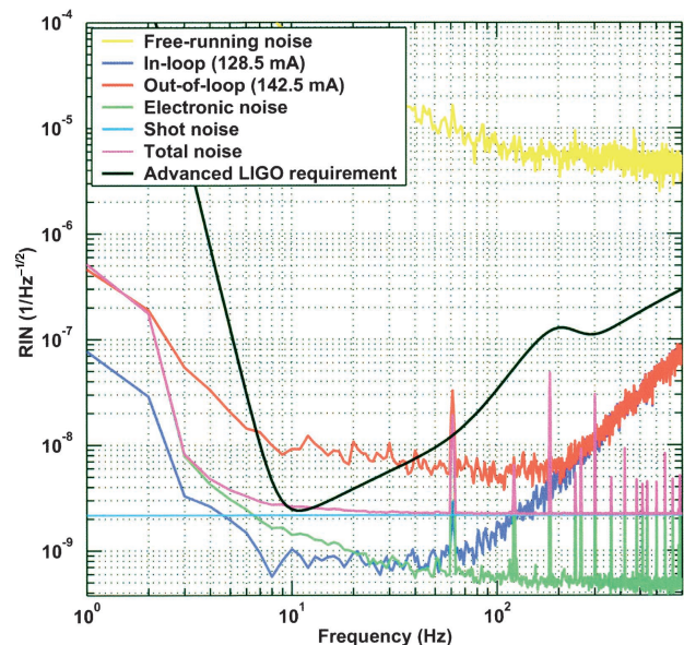
Fig. 1. Relative intensity noise (RIN) as measured by in-loop and out-of-loop photodetectors. The expected shot noise and measured electronic noise levels are shown in the light blue and green traces, respectively. The black curve shows the Advanced LIGO requirement. (Data taken June 29, 2003.)
