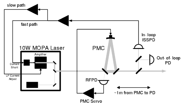
Fig. 2. Block diagram of the intensity stabilization servo. The fast path uses the fast CS actuator, whereas the slow path uses the low-bandwidth, high-range, LFCA. The control signal comes from the in-loop detector, and the out-of-loop detector is used for reference. RFPD, radio-frequency photodiode; PD, photodiode.
