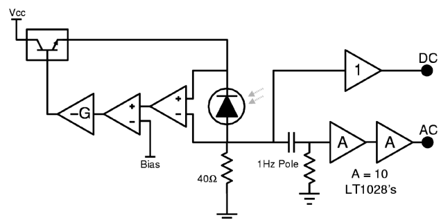
Fig. 3. Schematic of the photodiode circuit. The bias feedback control loop can be seen on the left and the preamplification on the right. 1, unity gain amplifier; G, inverting gain amplifier.
