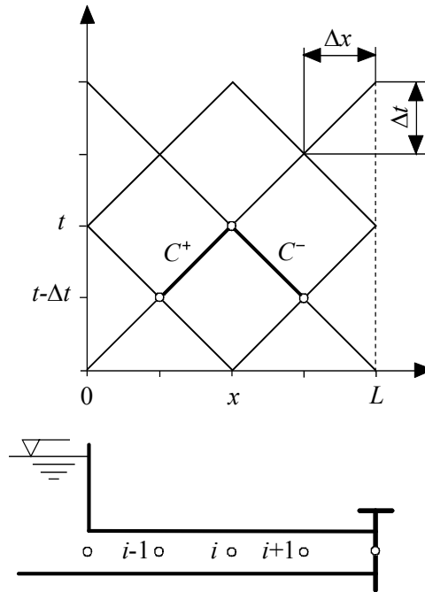
Figure 1 The method of characteristics staggered grid for a reservoir-pipe-valve system.
