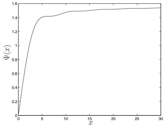
Figure 4: A plot of the function \Psi(x) (see equation (3.12)).
