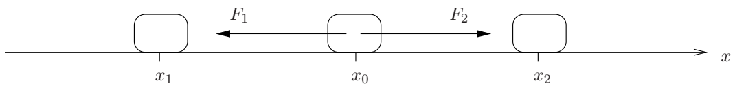
Figure 2: Forces F_1 and F_2 acting on a cell at x_0 due to attraction to cells at x_1 and x_2 respectively. When the cells are evenly spaced ( x_0 - x_1 = x_2 - x_0 ), the magnitudes of the forces are equal ( F_1 = F_2 ).
