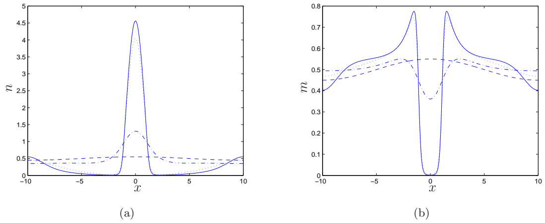
Figure 10: Numerical solution for cell densities n (a) and m (b) under Hypothesis 1 (see Table 1 ). Times shown: t = 0 (dash), t = 50 (dot-dash), t = 100 (dot) and t = 150 (solid). Parameter values: \chi_2 = 1 , \phi = 0.1 , \gamma_2 = 1 , D_n = D_m = 0.1 , R = 20 , r = 0.1 .
