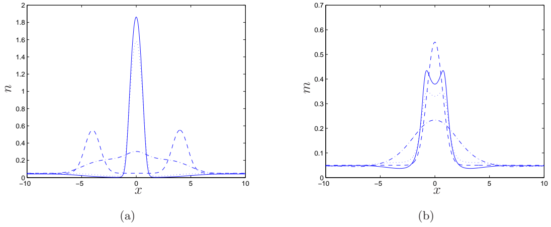
Figure 13: Numerical solution for cell densities n (a) and m (b) under Hypothesis 1 (see Table 1 ). Times shown: t = 0 (dash), t = 10 (dot-dash), t = 30 (dot) and t = 50 (solid). Parameter values: \chi_2 = 5 , \phi = 1 , \gamma_2 = 1 , D_n = D_m = 0.1 , R = 20 , r = 0.1 .
