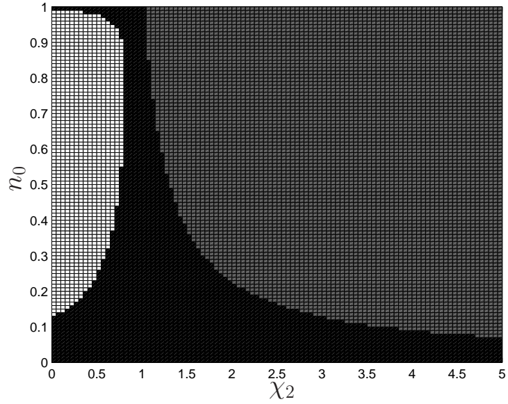
Figure 6: A plot of the stability regions for Hypothesis 1 (see Table 1 ). In black regions both roots of \omega are real and negative for all q , whilst dark grey denotes regions where complex conjugate roots can exist, but have negative real part. Hence in both the spatially homogeneous steady state is linearly stable to perturbations of all wavenumbers. In white regions the roots can be real and of differing sign (so the homogeneous state is linearly unstable to perturbations of certain wavenumbers). Parameter values: R = 100 , r = 0.1 , D_n = D_m = 0.1 , \phi = 0.1 , \gamma_2 = 1 , m_0 = 1 - n_0 .
