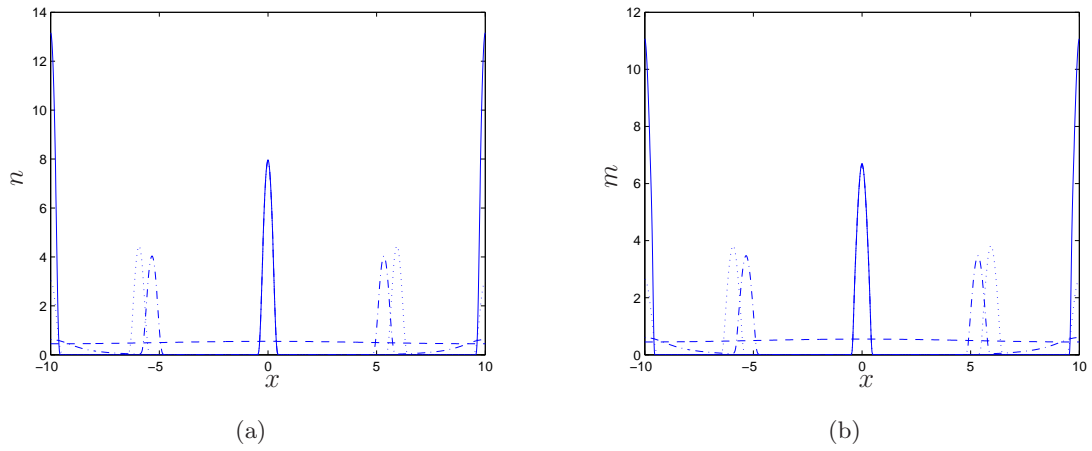
Figure 11: Numerical solution for cell densities n (a) and m (b) under Hypothesis 1 (see Table 1 ). Times shown: t = 0 (dash), t = 50 (dot-dash), t = 100 (dot) and t = 150 (solid). Parameter values: \chi_2 = 5 , \phi = 5 , \gamma_2 = 1 , D_n = D_m = 0.1 , R = 20 , r = 0.1 .
