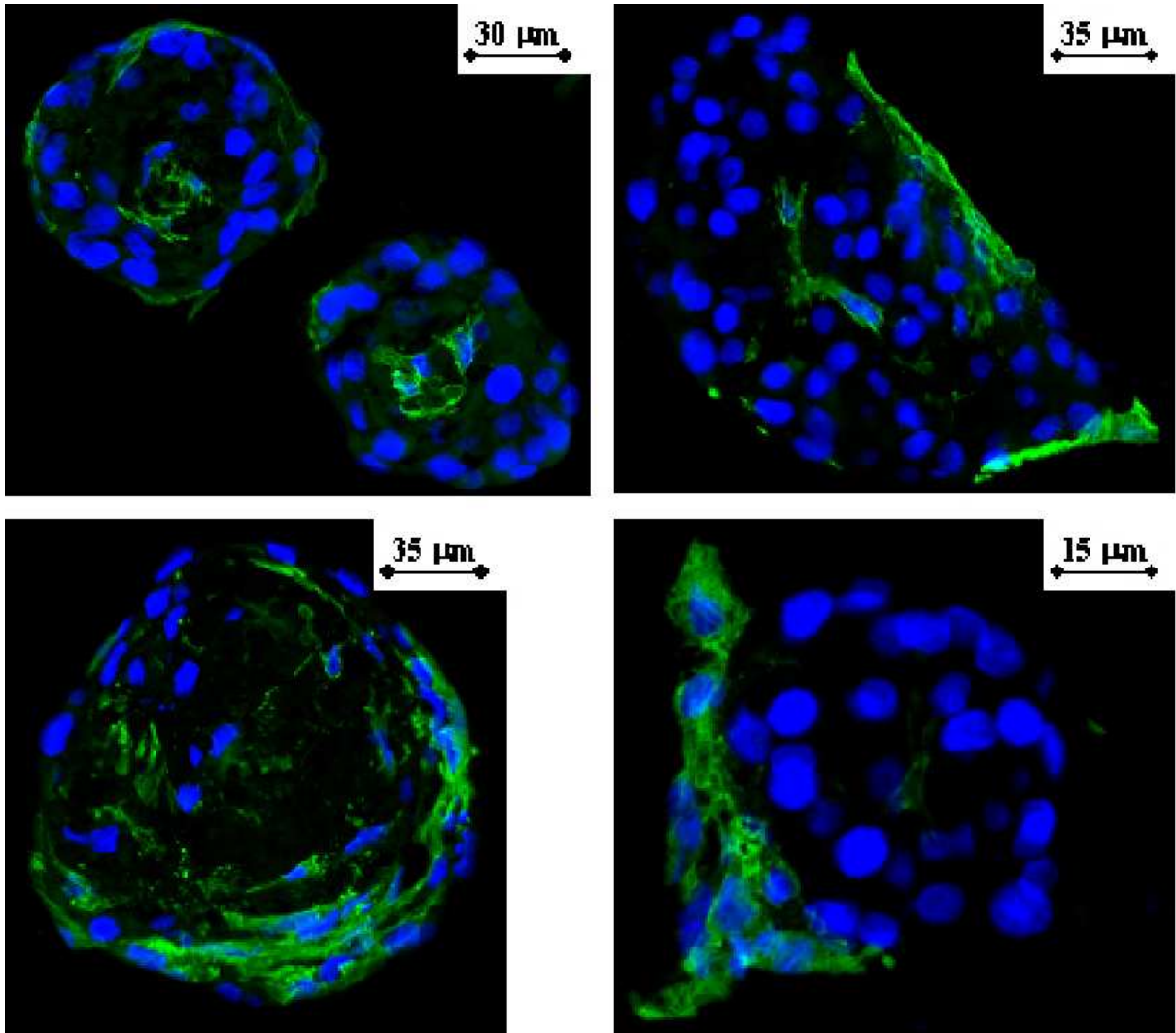
Figure 15: Sections through hepatocyte-stellate cell spheroids (reproduced from (Thomas et al., 2006)). Stellate cells appear green.
