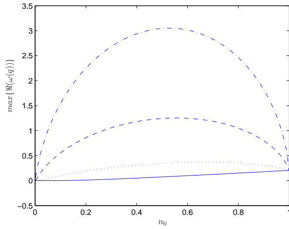
Figure 8: The dependence of maximum growth rate ( \max\{\Re(\omega(q))\} ) on the cell seeding density, n_0 for Hypothesis 1 (see Table 1 ), with m_0 = 1 - n_0 . Parameter values: \chi_2 = \phi = 0.5 (solid), \chi_2 = \phi = 2 (dot), \chi_2 = \phi = 5 (dash), \chi_2 = \phi = 10 (dot-dash) with \gamma_2 = 1 , R = 20 , r = 0.1 D_n = D_m = 0.1 in all cases.
