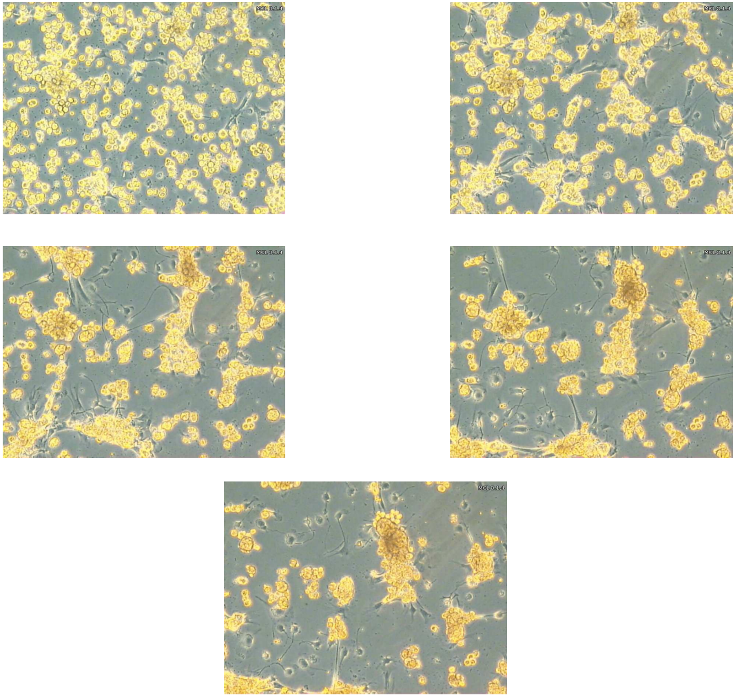
Figure 1: Snapshots from time-lapse video of an hepatocyte-stellate cell co-culture during aggregation. The hepatocytes appear yellow, and have a rounded morphology. Stellates appear grey, but their long cellular processes are clearly distinguishable. The images show an area approx 1000 \mu\text{m} \times 700 \mu\text{m} and were taken at approximately 5-hourly intervals (total time elapsed: approx. 21 hours). (Images courtesy of Robert Thomas, Tissue Engineering Group. Similar images, including later timepoints, are shown in (Thomas et al., 2006). Timelapse video footage is also available at: www.ecmjournal.org/journal/papers/vol011/vol011a03.php )
