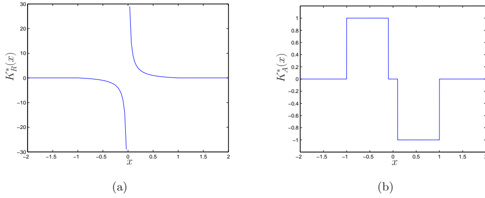
Figure 3: Sketches of the kernel functions used to describe repulsive and attractive cell-cell interactions respectively. (a) Repulsion kernel K_R^*(x) with R^* = r^* = 1 - see equation (2.3b). (b) Hepatocyte-stellate attraction kernel K_A^*(x) with A_2^* = a_2^* = 1, r^* = 0.1 - see equation (2.4d)
