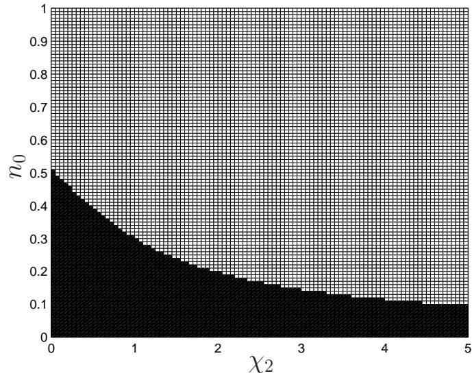
Figure 5: A plot of the stability regions for Hypothesis 1 (see Table 1 ), with R = 0 . Black (white) denotes regions for which the spatially homogeneous steady state is linearly stable (unstable) to perturbations of all (certain) wavenumbers. Parameter values: R = 0 , D_n = D_m = 0.5 , \phi = 0.5 , \gamma_2 = 1 , m_0 = 1 - n_0 .
