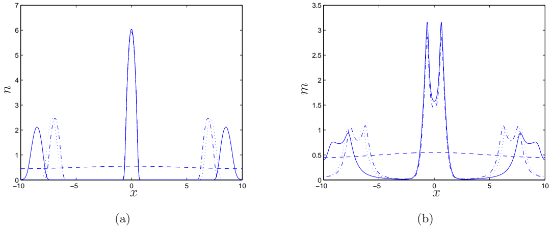
Figure 12: Numerical solution for cell densities n (a) and m (b) under Hypothesis 1 (see Table 1 ). Times shown: t = 0 (dash), t = 50 (dot-dash), t = 100 (dot) and t = 150 (solid). Parameter values: \chi_2 = 5 , \phi = 1 , \gamma_2 = 1 , D_n = D_m = 0.1 , R = 20 , r = 0.1 .
