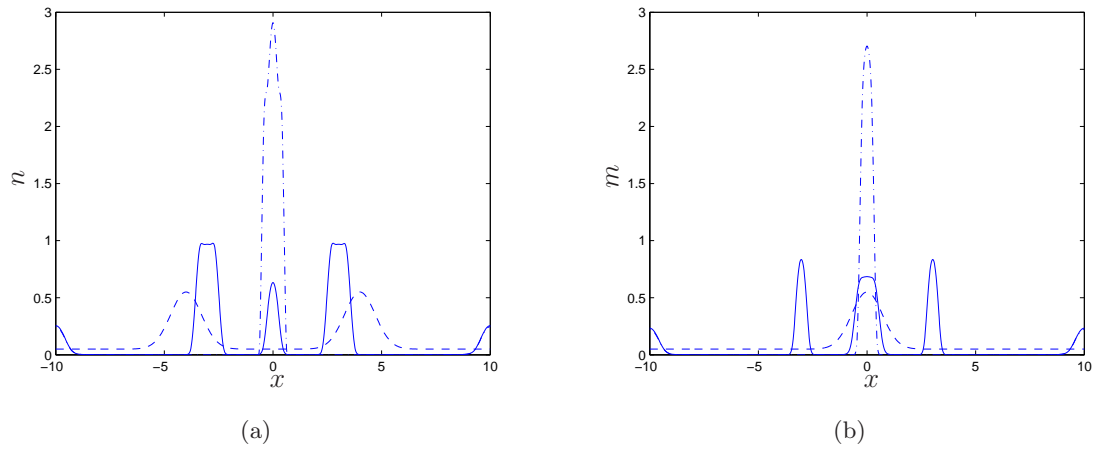
Figure 14: Numerical solution for cell densities n (a) and m (b) under Hypothesis 2 (see Table 1 ). Times shown: t = 0 (dash), t = 300 (solid) and t = 400 (dot-dash). Parameter values: A_2 = 5 , a_2 = 1 , D_n = D_m = 0.1 , R = 100 , r = 0.1 .
