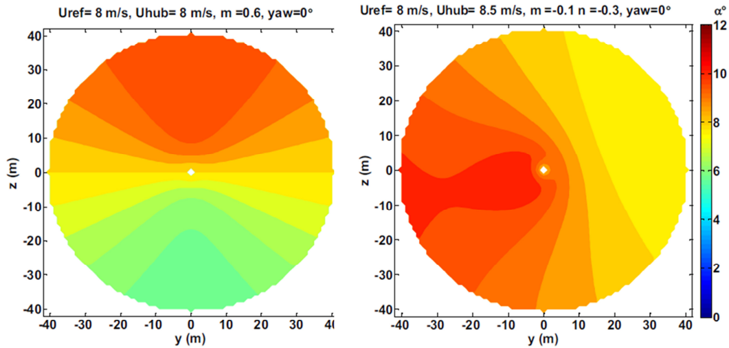
Figure 7 – Estimated variation in angle of attack due to wind shear; vertical (left) and combined horizontal and vertical (right) (Smith et al 2012)
