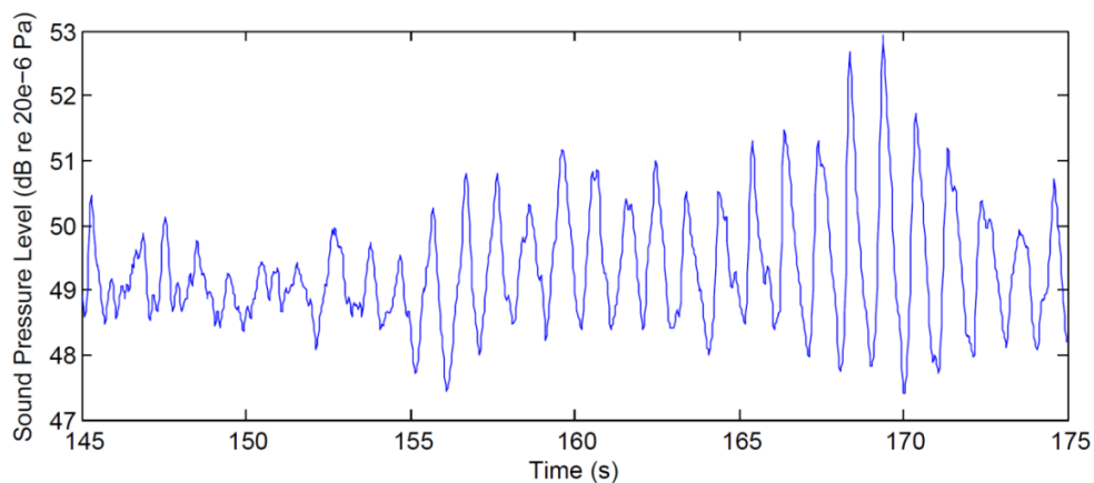
Figure 1 – Sound pressure level per 50ms due to Rhedes Park wind farm, measured at 750m from nearest turbine (adapted from Van den Berg 2004)
