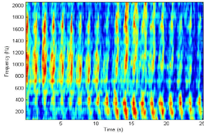
Figure 2 - Wind turbine spectrogram from 80m (Smith et al 2012)
