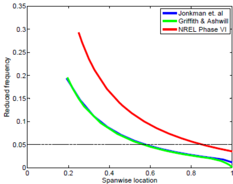
Figure 10 - Reduced frequency k vs span-wise location for several turbine blades
