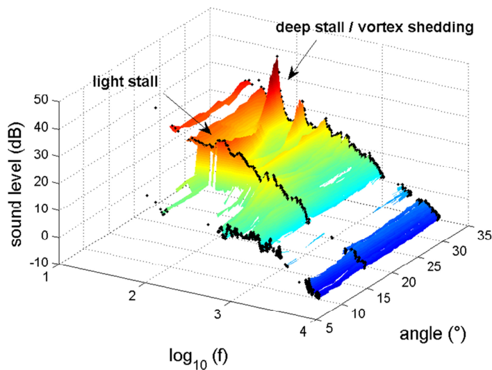
Figure 11 - Noise due to stall on a NACA 0012 airfoil at Re \sim 1.5 \times 10^5 (Moreau et al 2009)
