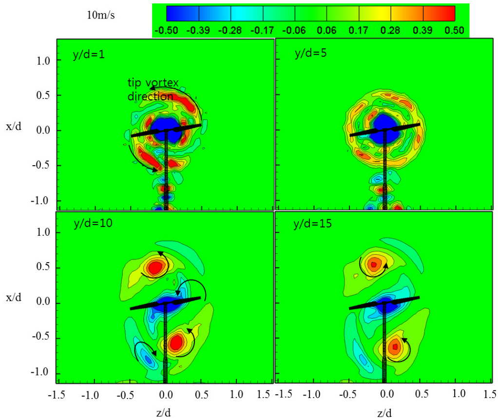
Figure 5– Simulated wake vortices in NREL experiment (adapted from Mo et al 2013)
