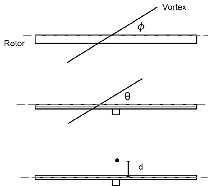
Figure 6 - Vortex orientation parameters. \phi : rotor-plane angle, \theta : shaft-plane angle, d : miss distance
