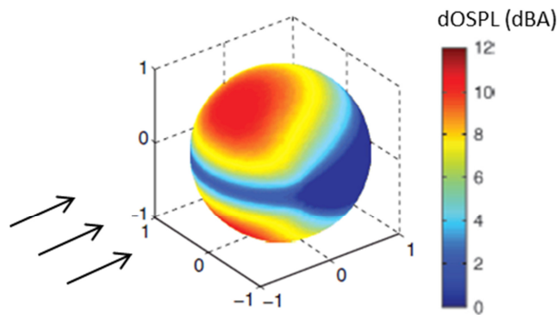
Figure 8 – Trailing-edge noise directivity (adapted from Oerlemans & Schepers 2009)
