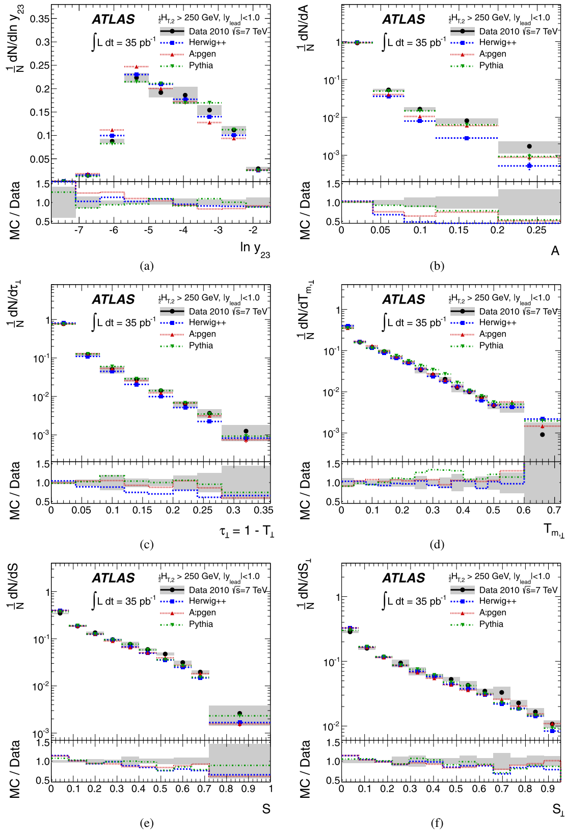
Fig. 2 Unfolded hadron-level distributions of the (a) third-jet resolution parameter, \ln y_{23} , (b) aplanarity, A, (c) transverse thrust, \tau_{\perp} , (d) minor component of the transverse thrust, T_{m,\perp} , (e) sphericity, S,
