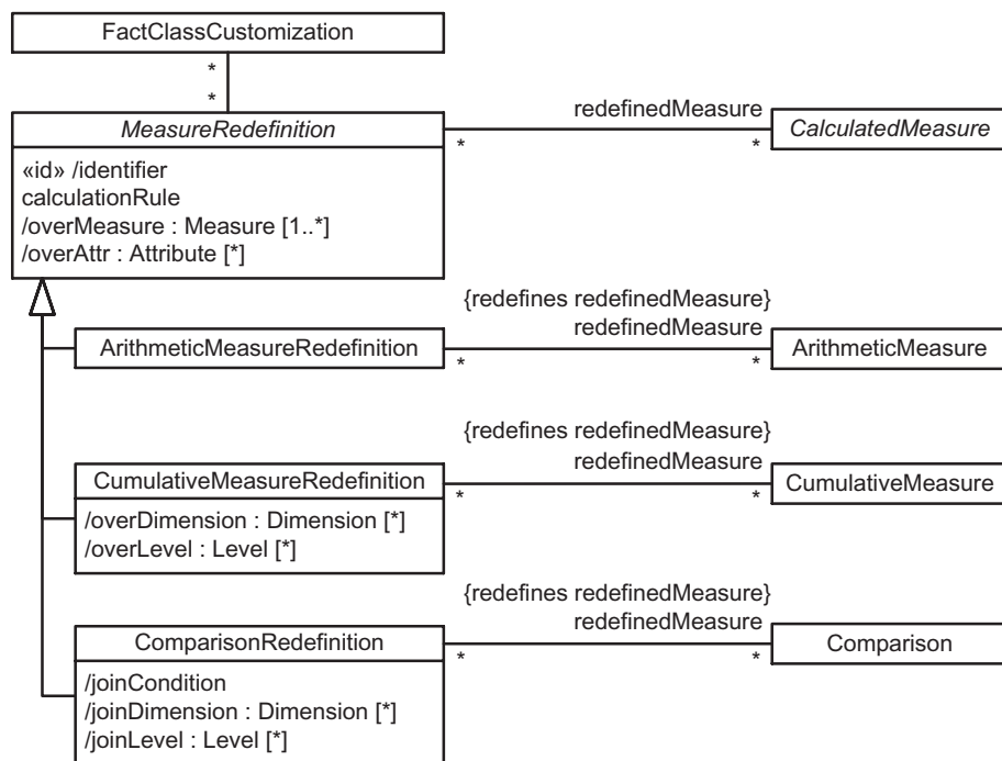
Fig. 7. Measure redefinitions in the metamodel of multidimensional reference models.
