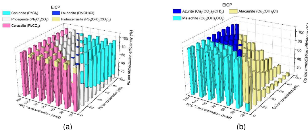
Figure 4. (a) variations of immobilization efficiency against hydrolyzed urea concentration and \text{Pb}^{2+} concentration under EICP and (b) variations of immobilization efficiency against hydrolyzed urea concentration and \text{Cu}^{2+} concentration under EICP
