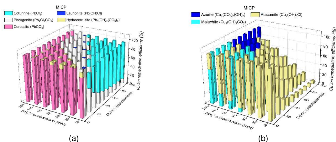
Figure 3. (a) variations of immobilization efficiency against hydrolyzed urea concentration and \text{Pb}^{2+} concentration under MICP and (b) variations of immobilization efficiency against hydrolyzed urea concentration and \text{Cu}^{2+} concentration under MICP
