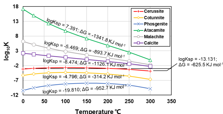
Figure 7. Relationships of \log_{10}K (thermodynamic equilibrium constant) versus temperature (in Celsius) against different carbonate precipitations applied to Pb and Cu immobilization
